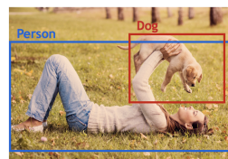
Object detection
