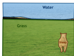
Image segmentation
