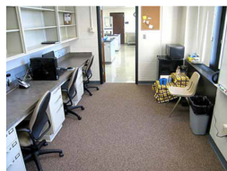
Object classification
