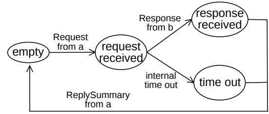
Figure 3: Basic Guaranteed Response protocol
