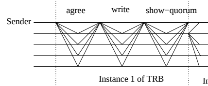
Figure 2: Terminating Reliable Broadcast (TRB) phases.
