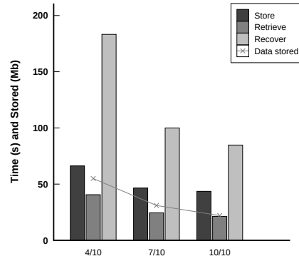
Figure 8: Operation time for 20MB at various encodings
