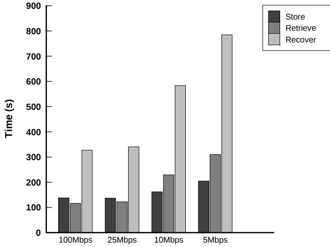
Figure 10: Operation under different network conditions
