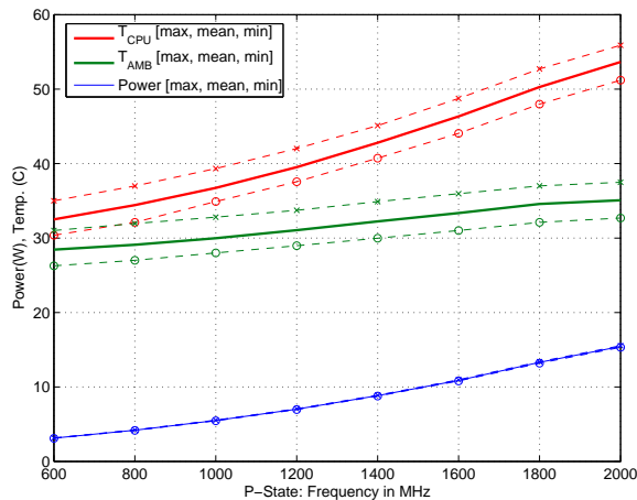
Figure 8: Steady-state power and temperature measurements for multiple invocations of daxy.
