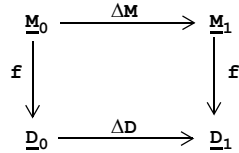
Figure 13. Commuting Diagram
