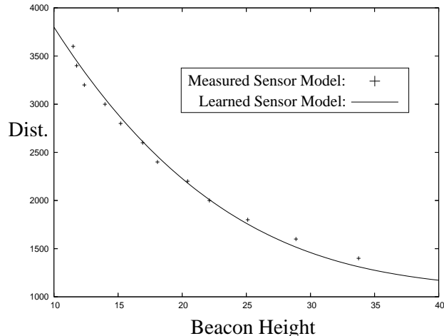
Fig. 4. The measured sensor model and a learned cubic model
