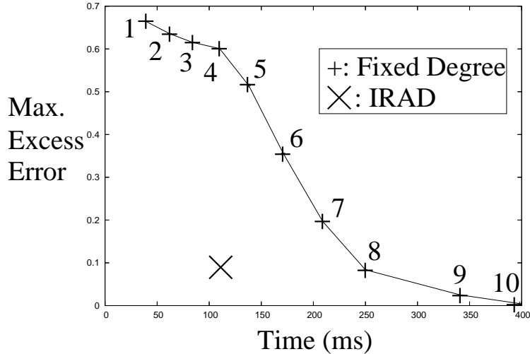
Fig. 2. The maximum excess errors and times attained by polynomial regression with a fixed degree, compared to PRAD.
