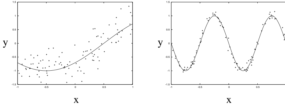
Fig. 1. Functions and 100 data points for two combinations of a and b , a = 2 and b = 8 (left), and a = 8 and b = 2 (right).
