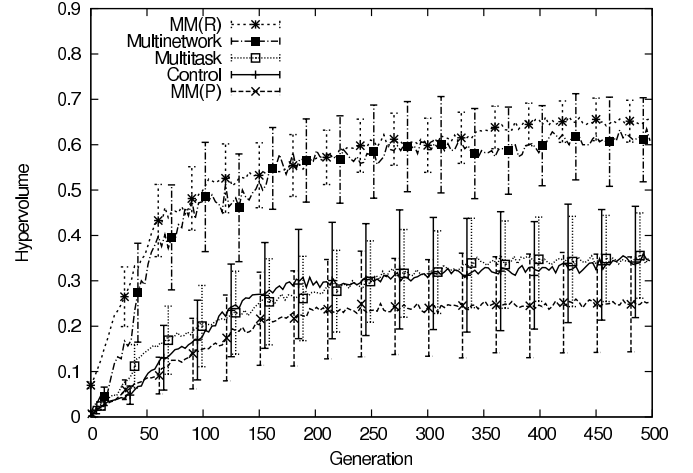
Fig. 12: Average hypervolumes in the Predator/Prey game. For each method, average hypervolumes across 20 runs are shown by generation with 95% confidence intervals. In contrast to the FBR game, MM(R) outperforms Control, MM(P), and Multitask significantly. None of these three methods with lower performance are significantly different from each other, though MM(P) is slightly below Control and Multitask, which are on roughly the same level. Multinetwork also significantly outperforms these three low performing methods, and by the end of evolution has an average hypervolume that is slightly lower, but not significantly different from, that of MM(R). This domain demonstrates a surprising failure of the Multitask approach, which should easily develop distinct behaviors for each task, and the impressive success of MM(R), which performs as well as if it could completely isolate both tasks, as Multinetwork does. This result thus demonstrates the potential power of discovering modes automatically.
