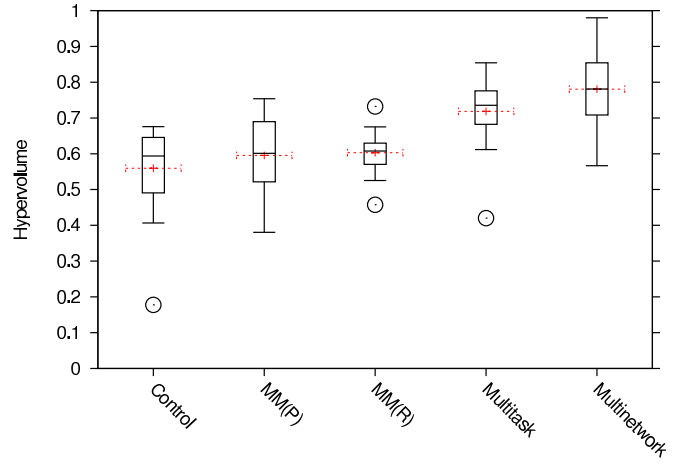
(a) Hypervolumes for Front Ramming.
