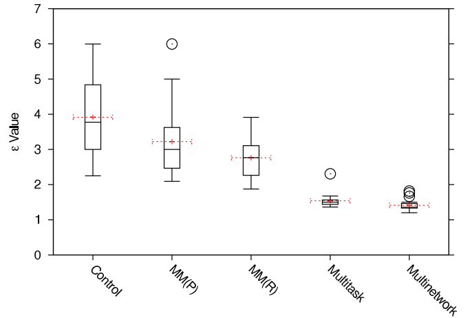
(a) I_{\epsilon}^1 Values.
