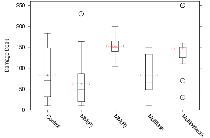
Fig. 14: Best damage-dealt scores in the Predator task of Predator/Prey. Isolating the Pareto fronts for the Predator task reduces it to a single-objective task. Because most individuals in the Pareto fronts for the full task had perfect damage-received and time-alive scores, these damage-dealt scores are primarily responsible for the differences in hypervolumes in the full task. The main reason that MM(R) is better than the other methods is that it always succeeds; it has no low scores at all. Most of the other methods have scores varying over a wider range, and thus much lower averages and medians. The only exception is Multinetwork, which, despite some low outliers, has very high median and average performance. It is particularly surprising that the lowest scores in the other methods can be so low. The pressure to perform well in the Prey task is clearly a big distraction to these other methods, and sometimes leads the evolving populations in a one-way direction away from good performance in the Predator task.
