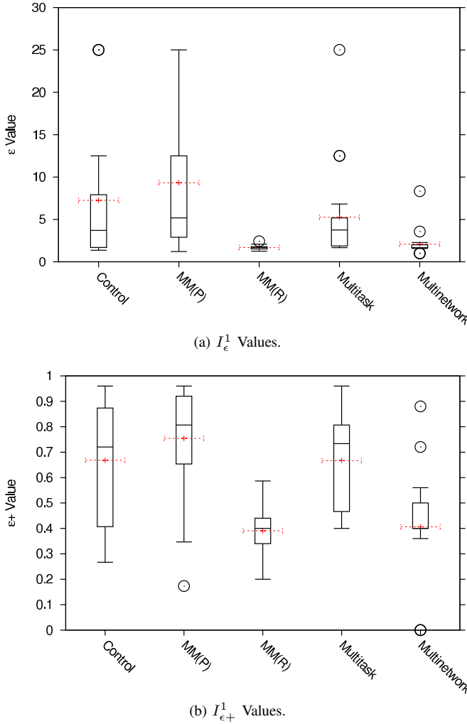
Fig. 13: Epsilon indicator values in the final generation of Predator/Prey. Given the final Pareto fronts for each of the 20 runs with each method, the (a) I_{\epsilon}^1 values, and (b) I_{\epsilon}^+ values are calculated, and presented in the same manner as in Fig. 5. MM(R) and Multinetwork are superior to all other methods. MM(R)'s performance is unexpected since Multitask, like Multinetwork, always has knowledge of the current task, and has a specific policy for each task. There is little difference between Control, Multitask, and MM(P). In terms of I_{\epsilon}^1 values, Control and Multitask seem better than MM(P), but Table V indicates that these differences are not significant. The slight difference between MM(R) and Multinetwork is not significant either.
