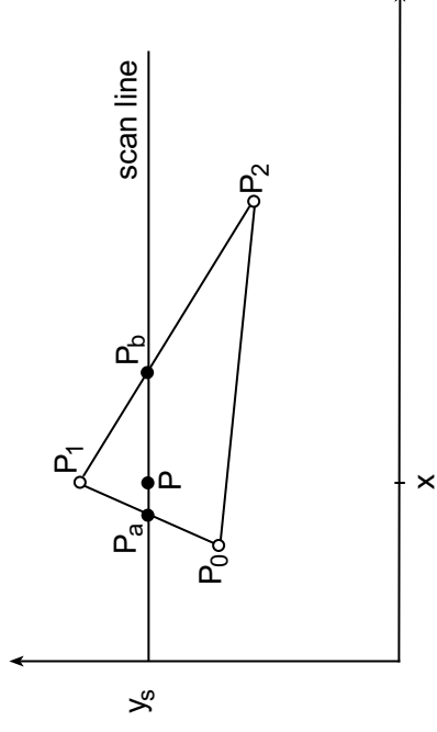
Depth-buffer interpolation.
