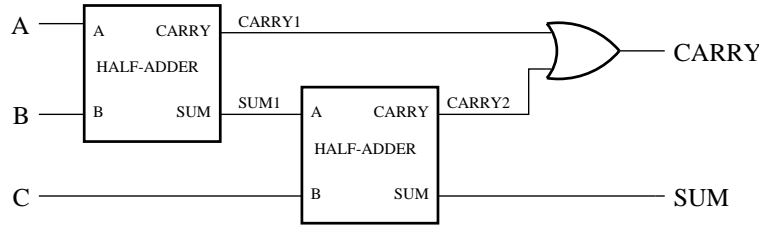
Figure 4: Full-Adder Circuit
