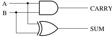
Figure 3: Half-Adder Circuit
