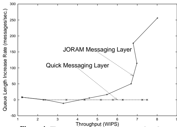
Figure 4: The growth rate of message queue length.
