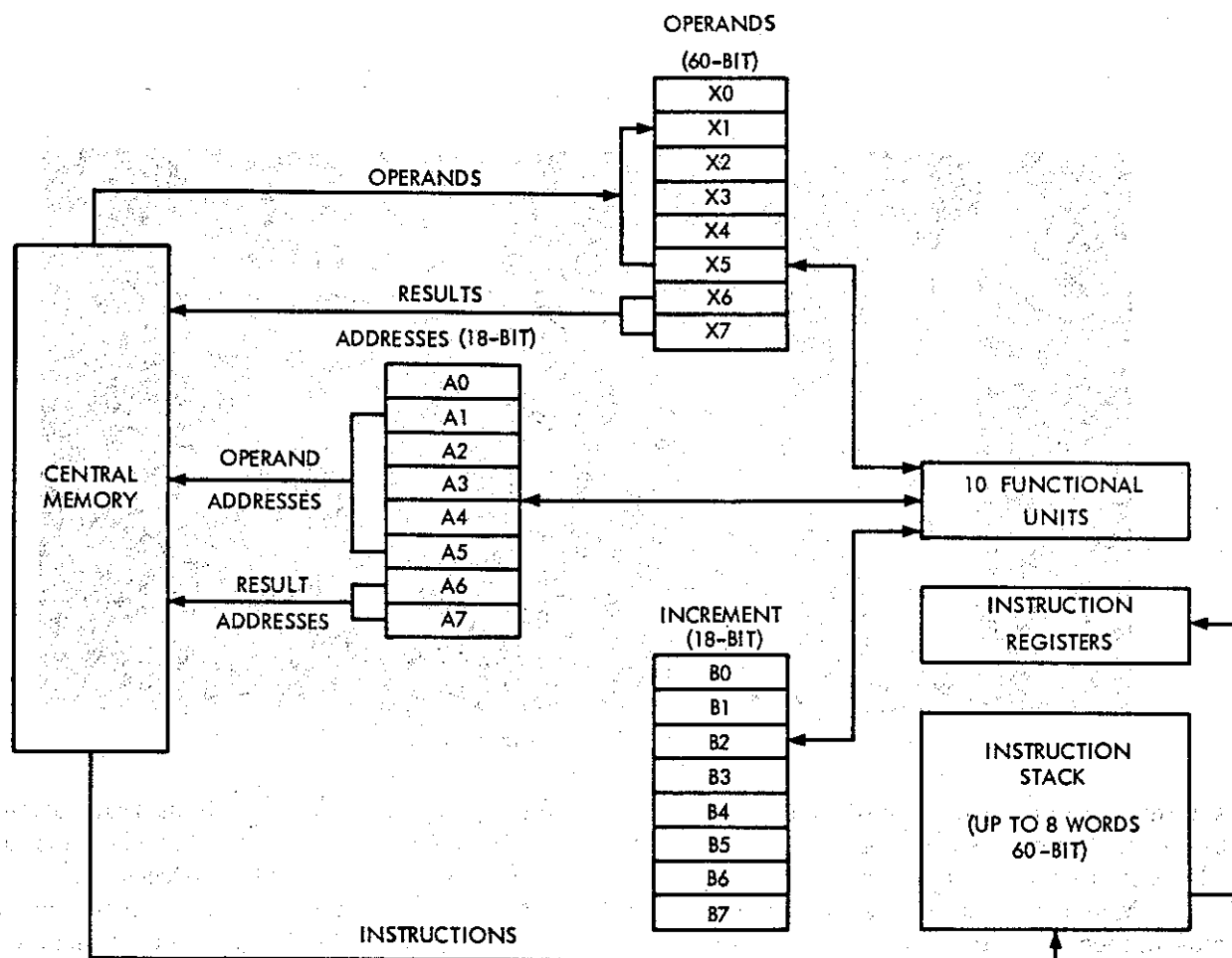
Figure 6. Central Processor Operating Registers.
