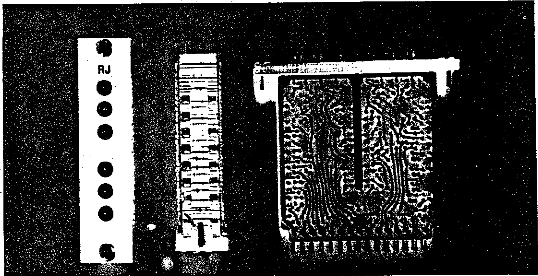
Figure 7. 6600 Printed Circuit Module.
