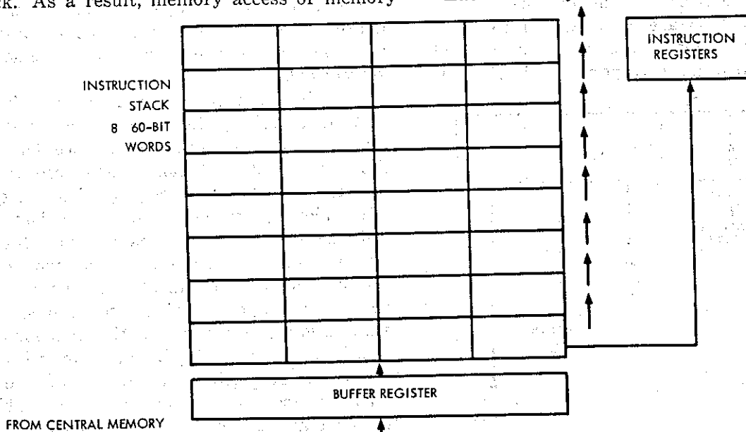
Figure 5. 6600 Instruction Stack Operation.
