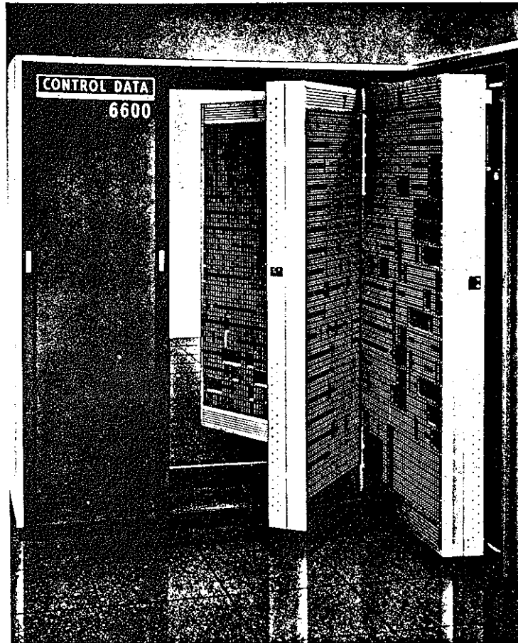
Figure 9. 6600 Main Frame Section.
