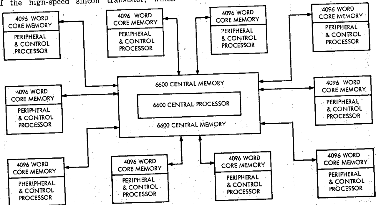
Figure 1. Control Data 6600.
