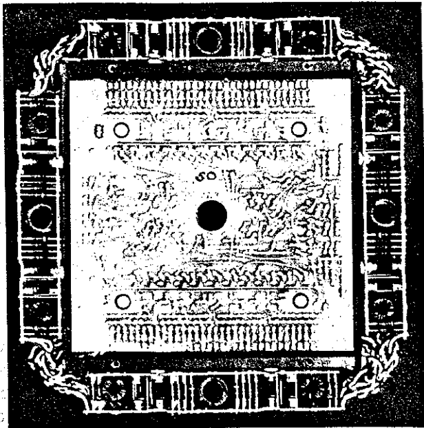
Figure 8. 6600 Memory Module.
