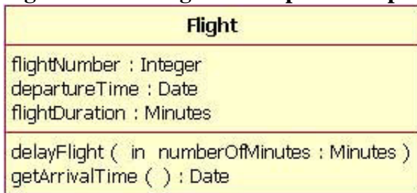
Figure 3: The Flight class operations parameters include the optional "in" marking
