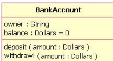
Figure 2: A Bank Account class diagram showing the balance attribute's value defaulted to zero dollars
