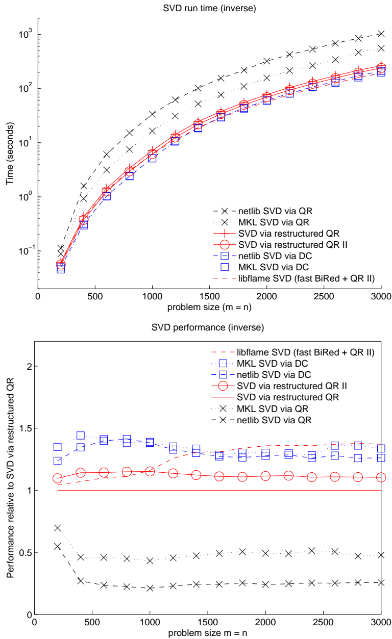
Fig. 32. Top: Run times for various implementations of SVD. Bottom: Performance of implementations relative to SVD via restructured QR. Experiments were run with complex matrices generated with inverse distributions of singular values. Here, the problem sizes listed are m = n . In the case of “SVD via restructured QR” and “SVD via restructured QR II”, matrices were reduced to bidiagonal form using a conventional implementation similar to that of zgebrd . Results for “libflame SVD (fast BiRed + QR II)” combine the higher-performing bidiagonal reduction presented in [Van Zee et al. 2011] with the restructured QR II algorithm.
