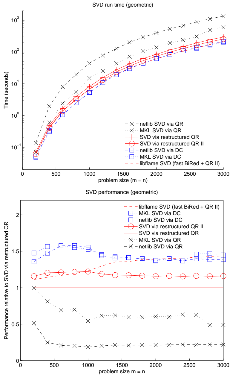
Fig. 31. Top: Run times for various implementations of SVD. Bottom: Performance of implementations relative to SVD via restructured QR. Experiments were run with complex matrices generated with geometric distributions of singular values. Here, the problem sizes listed are m = n . In the case of “SVD via restructured QR” and “SVD via restructured QR II”, matrices were reduced to bidiagonal form using a conventional implementation similar to that of zgebrd . Results for “libflame SVD (fast BiRed + QR II)” combine the higher-performing bidiagonal reduction presented in [Van Zee et al. 2011] with the restructured QR II algorithm.
