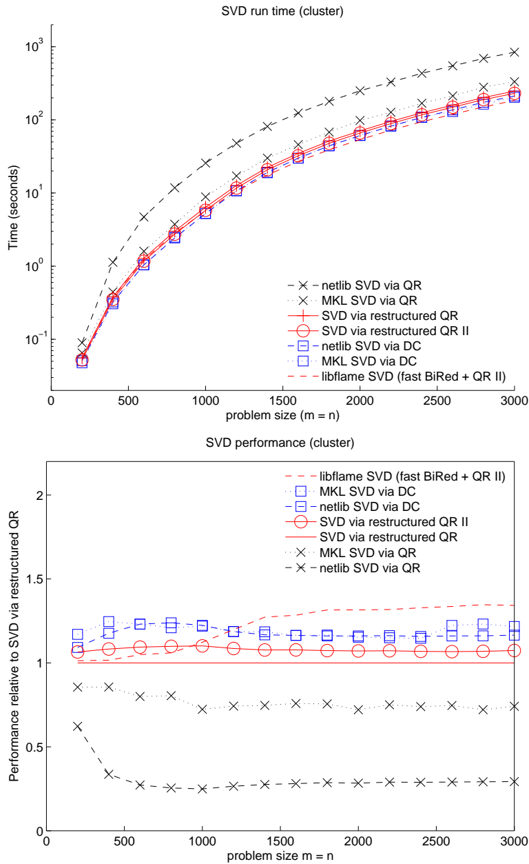
Fig. 30. Top: Run times for various implementations of SVD. Bottom: Performance of implementations relative to SVD via restructured QR. Experiments were run with complex matrices generated with clustered distributions of singular values. Here, the problem sizes listed are m = n . In the case of “SVD via restructured QR” and “SVD via restructured QR II”, matrices were reduced to bidiagonal form using a conventional implementation similar to that of zgebrd . Results for “libflame SVD (fast BiRed + QR II)” combine the higher-performing bidiagonal reduction presented in [Van Zee et al. 2011] with the restructured QR II algorithm.
