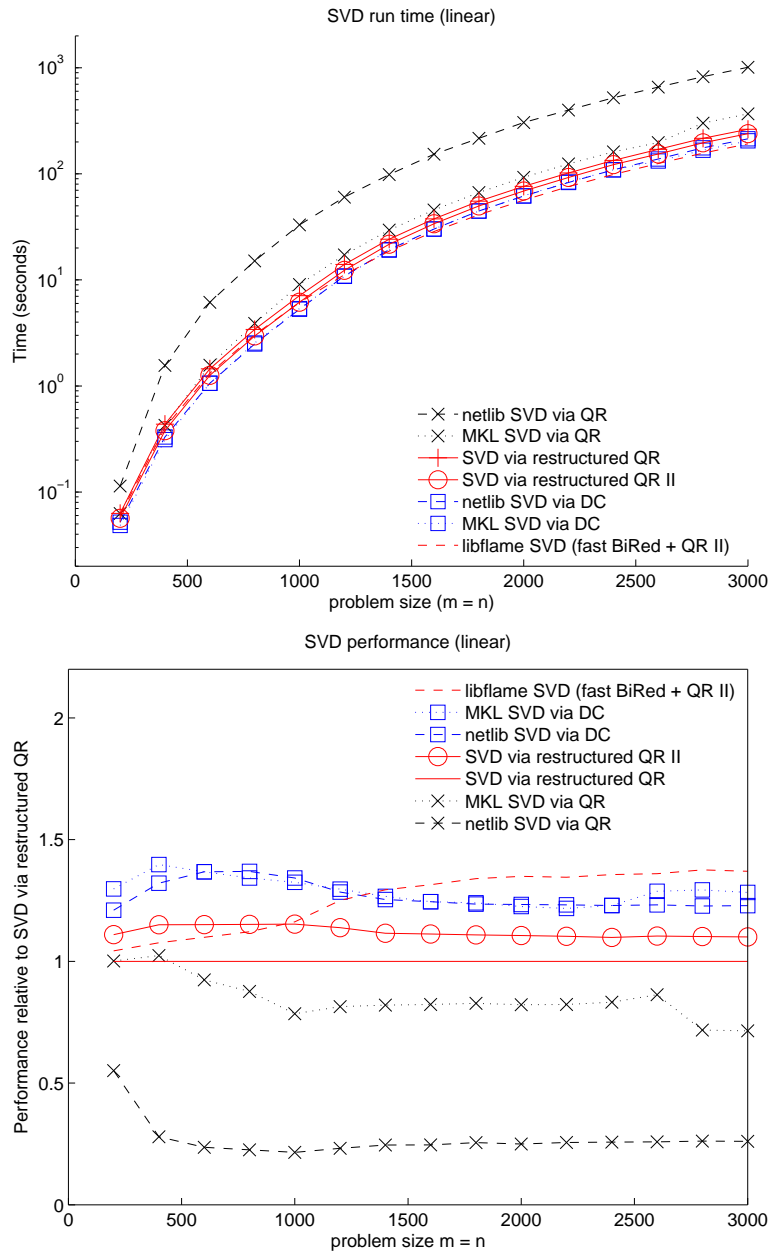
Fig. 33. Top: Run times for various implementations of SVD. Bottom: Performance of implementations relative to SVD via restructured QR. Experiments were run with complex matrices generated with linear distributions of singular values. Here, the problem sizes listed are m = n . In the case of “SVD via restructured QR” and “SVD via restructured QR II”, matrices were reduced to bidiagonal form using a conventional implementation similar to that of zgebrd . Results for “libflame SVD (fast BiRed + QR II)” combine the higher-performing bidiagonal reduction presented in [Van Zee et al. 2011] with the restructured QR II algorithm.
