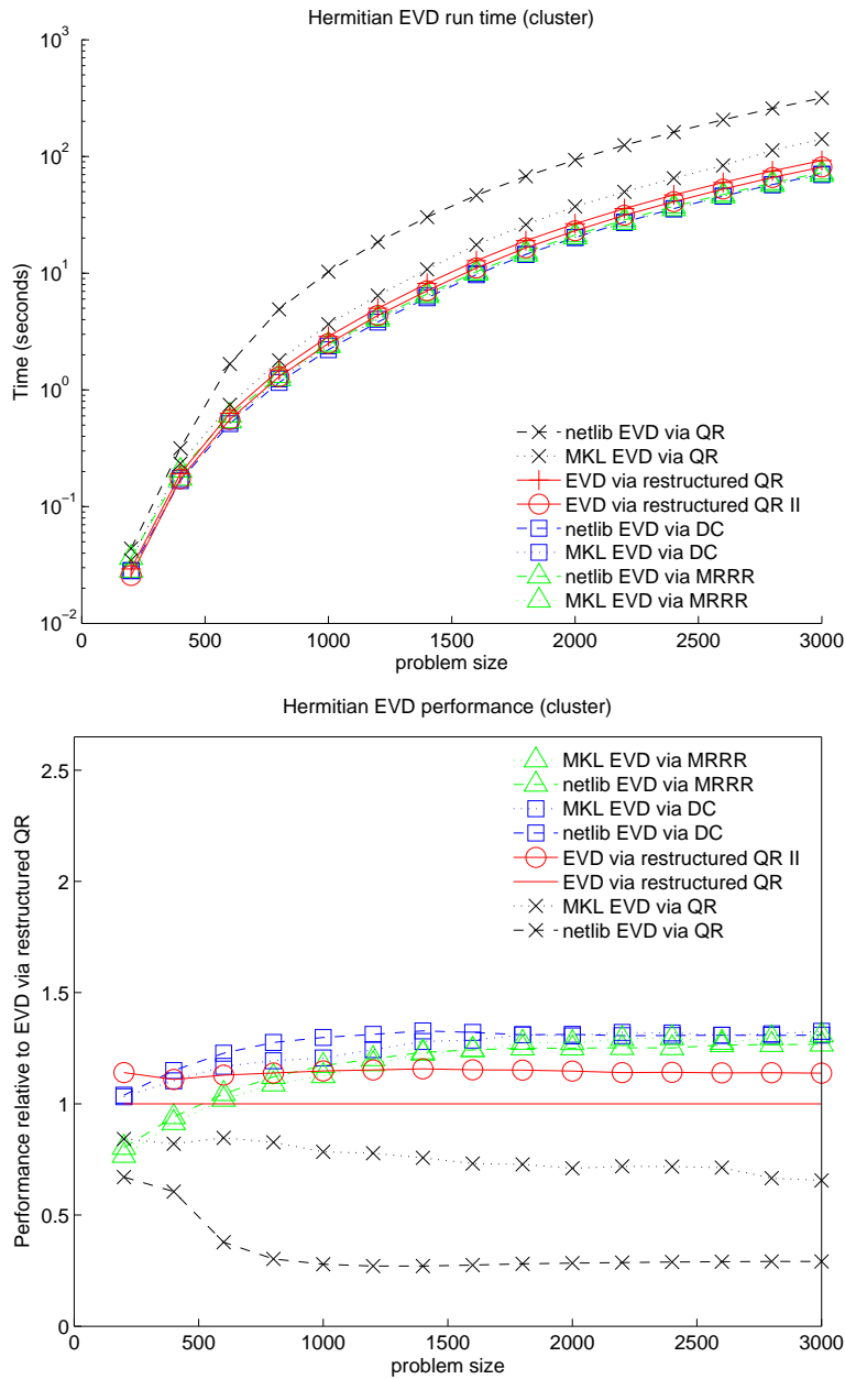
Fig. 24. Top: Run times for various implementations of Hermitian EVD. Bottom: Performance of implementations relative to EVD via restructured QR. Experiments were run with complex matrices generated with clustered distributions of eigenvalues. In the case of EVD via restructured QR, matrices were reduced to tridiagonal form using a conventional implementation similar to that of zhetrd .
