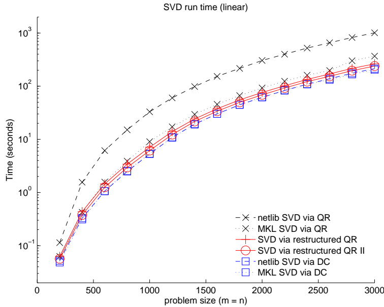
Fig. 20. Run times for various implementations of SVD. Experiments were run with complex matrices generated with linear distributions of singular values. Here, the problem sizes listed are m = n .
