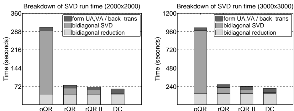
Fig. 21. Breakdown of time spent in the three stages of SVD: bidiagonal reduction, bidiagonal SVD, and the formation of U_A and V_A (for QR-based algorithms) or the back-transformation (netlib D&C) for problem sizes of 2000 \times 2000 (left) and 3000 \times 3000 (right). Here, “oQR” refers to EVD based on the original netlib QR algorithm while “rQR” refers to our restructured algorithm. This shows how the run time advantage of the bidiagonal D&C algorithm over restructured QR is partially negated by increased time spent in the former method’s back-transformations.
