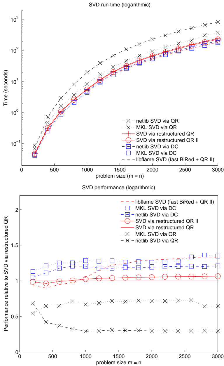
Fig. 34. Top: Run times for various implementations of SVD. Bottom: Performance of implementations relative to SVD via restructured QR. Experiments were run with complex matrices generated with logarithmic distributions of singular values. Here, the problem sizes listed are m = n . In the case of “SVD via restructured QR” and “SVD via restructured QR II”, matrices were reduced to bidiagonal form using a conventional implementation similar to that of zgebrd . Results for “libflame SVD (fast BiRed + QR II)” combine the higher-performing bidiagonal reduction presented in [Van Zee et al. 2011] with the restructured QR II algorithm.
