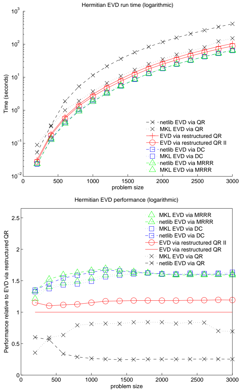
Fig. 28. Top: Run times for various implementations of Hermitian EVD. Bottom: Performance of implementations relative to EVD via restructured QR. Experiments were run with complex matrices generated with logarithmic distributions of eigenvalues. In the case of EVD via restructured QR, matrices were reduced to tridiagonal form using a conventional implementation similar to that of zhetrd .
