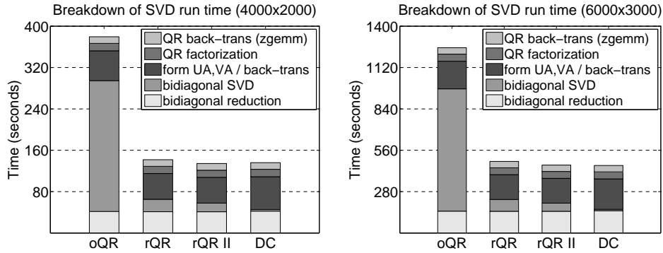
Fig. 23. Breakdown of time spent in the three stages of SVD: bidiagonal reduction, bidiagonal SVD, and the formation of U_A and V_A (for QR-based algorithms) or the back-transformation (netlib D&C) for problem sizes of 4000 \times 2000 (left) and 6000 \times 3000 (right). Here, “oQR” refers to EVD based on the original netlib QR algorithm while “rQR” refers to our restructured algorithm. In contrast to Figure 21, these graphs reflect the additional time spent in the QR factorization of A and the corresponding backtransformation necessary to combine Q with U_R U_B , which is implemented via zgemm .
