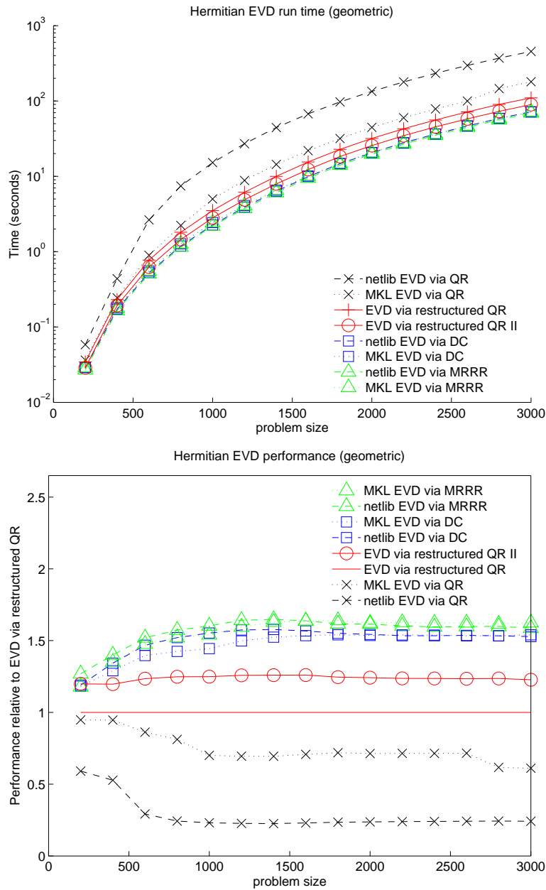
Fig. 25. Top: Run times for various implementations of Hermitian EVD. Bottom: Performance of implementations relative to EVD via restructured QR. Experiments were run with complex matrices generated with geometric distributions of eigenvalues. In the case of EVD via restructured QR, matrices were reduced to tridiagonal form using a conventional implementation similar to that of zhetrd .
