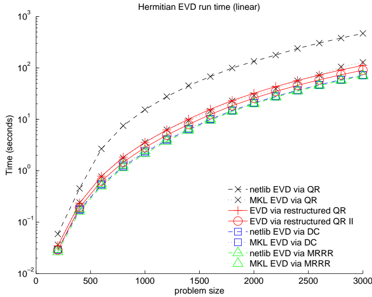
Fig. 18. Run times for various implementations of Hermitian EVD. Experiments were run with complex matrices generated with linear distributions of eigenvalues.
