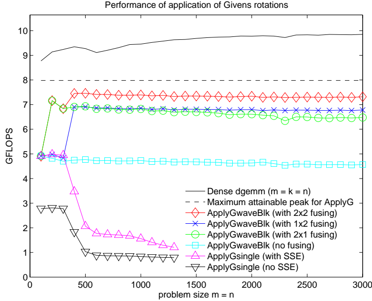
Fig. 17. Performance of various implementations for applying k = 192 sets of Givens rotations. Those implementations based on blocked algorithms use an algorithmic blocksize b = 256 . The maximum attainable peak for applying Givens rotations, which is 25% lower than that of dgemm because of a 1:2 ratio of floating-point additions to multiplications, is also shown. Performance results for dgemm , where all matrix dimensions are equal, are included for reference.
