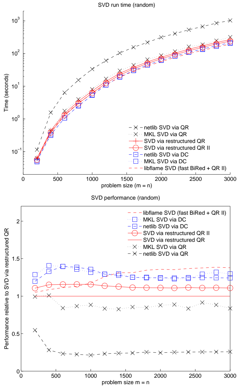
Fig. 35. Top: Run times for various implementations of SVD. Bottom: Performance of implementations relative to SVD via restructured QR. Experiments were run with complex matrices generated with random distributions of singular values. Here, the problem sizes listed are m = n . In the case of “SVD via restructured QR” and “SVD via restructured QR II”, matrices were reduced to bidiagonal form using a conventional implementation similar to that of zgebrd . Results for “libflame SVD (fast BiRed + QR II)” combine the higher-performing bidiagonal reduction presented in [Van Zee et al. 2011] with the restructured QR II algorithm.
