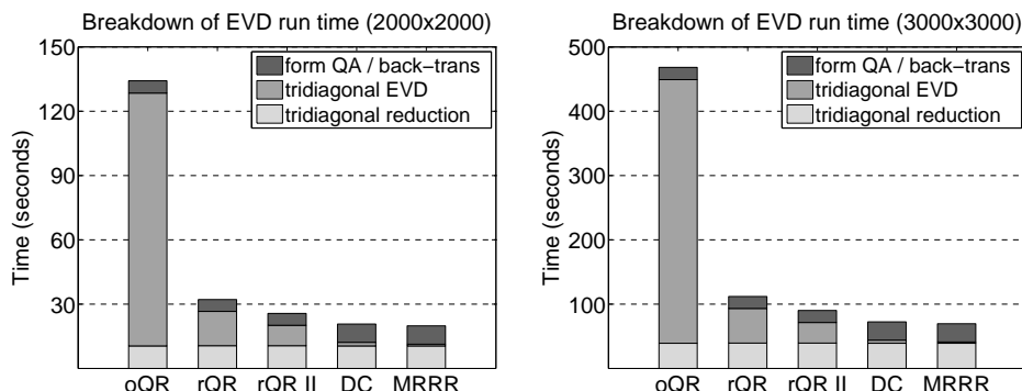
Fig. 19. Breakdown of time spent in the three stages of Hermitian EVD: tridiagonal reduction, tridiagonal EVD, and the formation of Q_A (for QR-based algorithms) or the back-transformation (netlib D&C and MRRR) for problem sizes of 2000 \times 2000 (left) and 3000 \times 3000 (right). Here, “oQR” refers to EVD based on the original netlib QR algorithm while “rQR” refers to our restructured algorithm. This shows how the run time advantage of the tridiagonal D&C and MRRR algorithms over restructured QR is partially negated by increased time spent in the former methods’ back-transformations.
