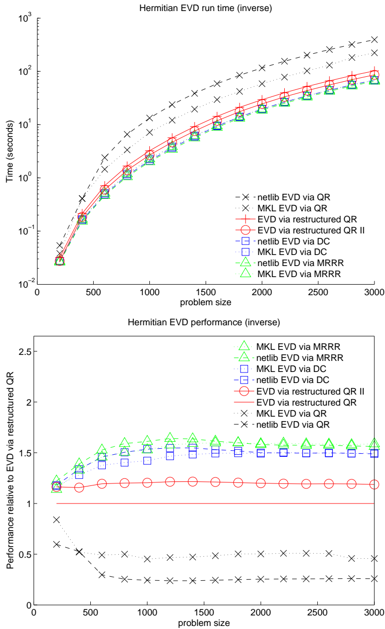
Fig. 26. Top: Run times for various implementations of Hermitian EVD. Bottom: Performance of implementations relative to EVD via restructured QR. Experiments were run with complex matrices generated with inverse distributions of eigenvalues. In the case of EVD via restructured QR, matrices were reduced to tridiagonal form using a conventional implementation similar to that of zhetrd.
