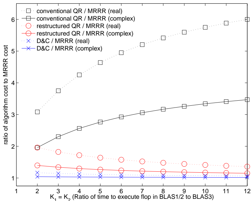
Fig. 3. Predicted ratios of floating-point operation cost for various eigenvalue algorithms relative to the cost of Hermitian eigenvalue decomposition via MRRR.
