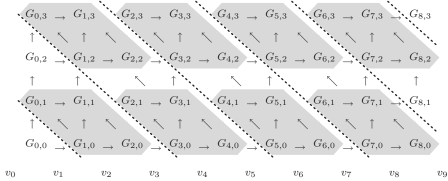
Fig. 14. Combining the approaches from Figures 12 and 13, we can fuse in both the k and n dimensions. This creates parallelogram-shaped groups of fusings. This two-dimensional fusing reduces the average number of column-access memory operations per rotation from four, in an algorithm that uses no fusing, to just two.
