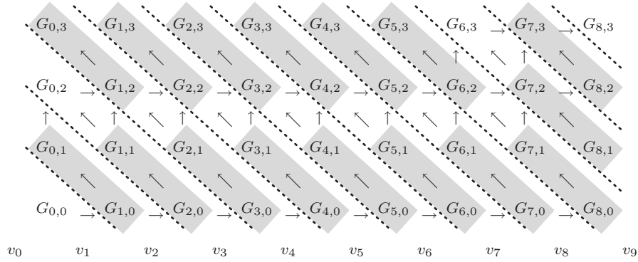
Fig. 12. By fusing pairs of successive rotations within the same wave, the number of memory operations performed on each element of V , per rotation applied, may be reduced from approximately four to three. Here, fused rotations are highlighted, with arrows redrawn to show dependencies within a fused pair as well as dependencies between pairs. Rotation pairs may be applied in waves, similar to the approach illustrated by Figure 4. Note that the updated dependencies satisfy the original dependency graph.
