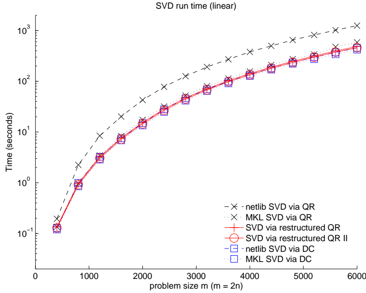
Fig. 22. Run times for various implementations of SVD. Experiments were run with complex matrices generated with linear distributions of singular values. Here, the problem sizes listed are m , where m = 2n .
