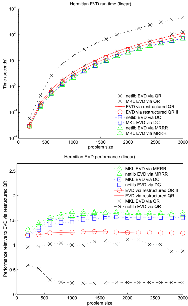
Fig. 27. Top: Run times for various implementations of Hermitian EVD. Bottom: Performance of implementations relative to EVD via restructured QR. Experiments were run with complex matrices generated with linear distributions of eigenvalues. In the case of EVD via restructured QR, matrices were reduced to tridiagonal form using a conventional implementation similar to that of zhetrd.
