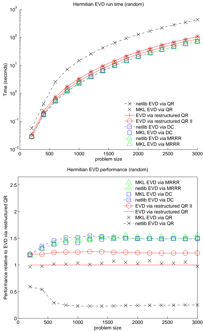
Fig. 29. Top: Run times for various implementations of Hermitian EVD. Bottom: Performance of implementations relative to EVD via restructured QR. Experiments were run with complex matrices generated with random distributions of eigenvalues. In the case of EVD via restructured QR, matrices were reduced to tridiagonal form using a conventional implementation similar to that of zhetrd.
