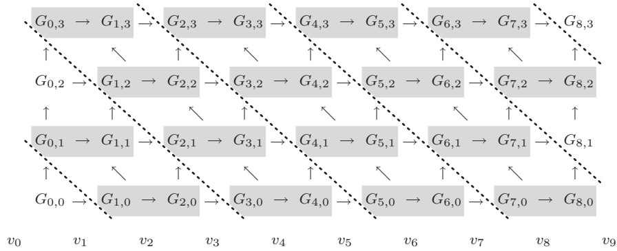
Fig. 13. Instead of fusing successive rotations within the same wave, as shown in Figure 12, we may also fuse pairs of successive rotations from the same Francis step. This approach similarly reduces the number of memory operations performed on each element of V per rotation from four to three.
