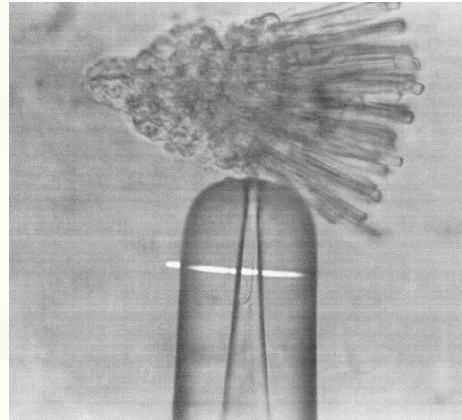
Measuring photoreceptor photocurrent (Wandell, 4.15)
