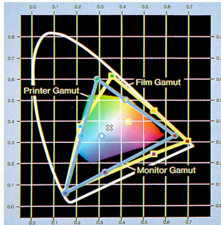
Gamuts of a few common output devices in CIE space (Foley, II.2)
