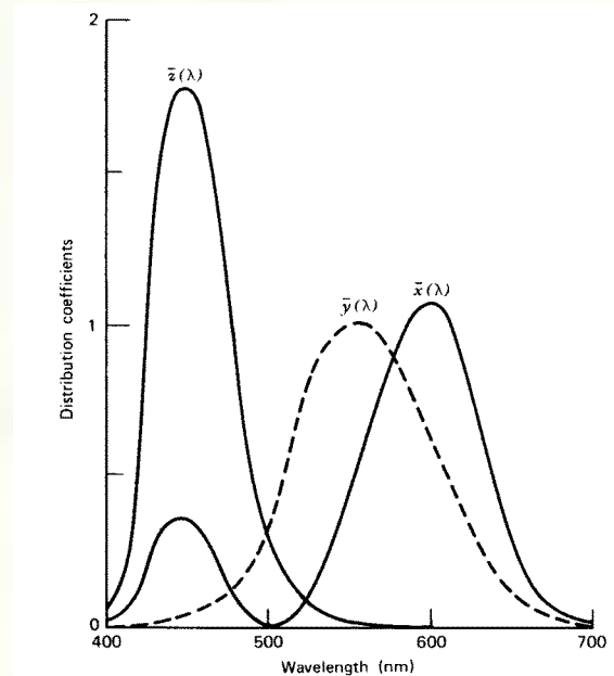
The XYZ color matching functions (Wasserman 3.8)
