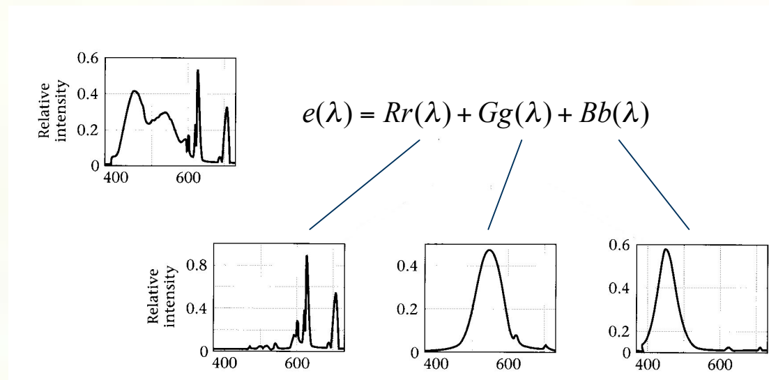
Emission spectra for RGB monitor phosphors (Wandell B.3)
