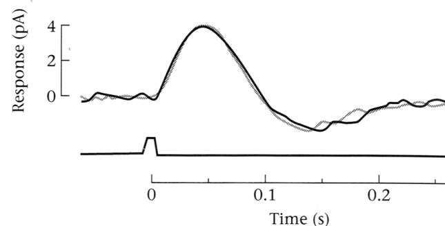
Photocurrents measured for two light stimuli: 550nm (solid) and 659 nm (gray). The brightnesses of the stimuli are different, but the shape of the response is the same. (Wandell 4.17)
