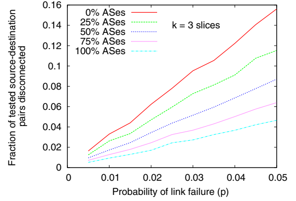
Figure 13: BGP Splicing: Incremental deployment.
