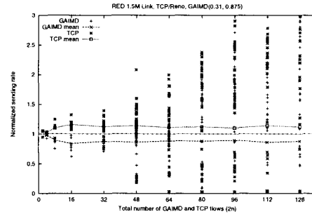
Figure 15. Normalized sending rates for 1.5Mbps RED link with Reno
