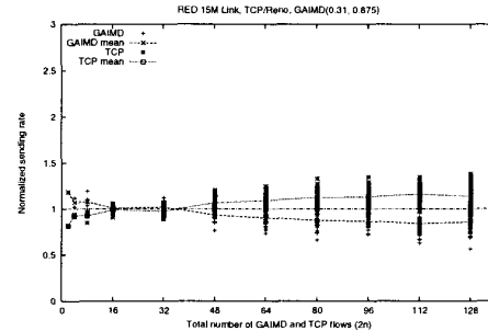
Figure 16. Normalized sending rates for 15Mbps RED link with Reno
