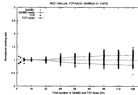
Figure 20. Normalized sending rates for 15Mbps RED link with TCP SACK
