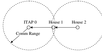
FIGURE 1. A linear topology with 2 houses.
