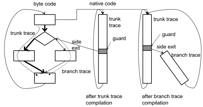
Figure 1. Byte code and native code transition in the trace-based JIT. Initially, the interpreter interprets on the byte code. First detected hot path (thick path) is traced forming a trunk trace. Following hot paths guarded and installed in a side-exit. The compiler attach the branch trace, which begins from the hot side-exit to the loop header, to the trunk trace.
