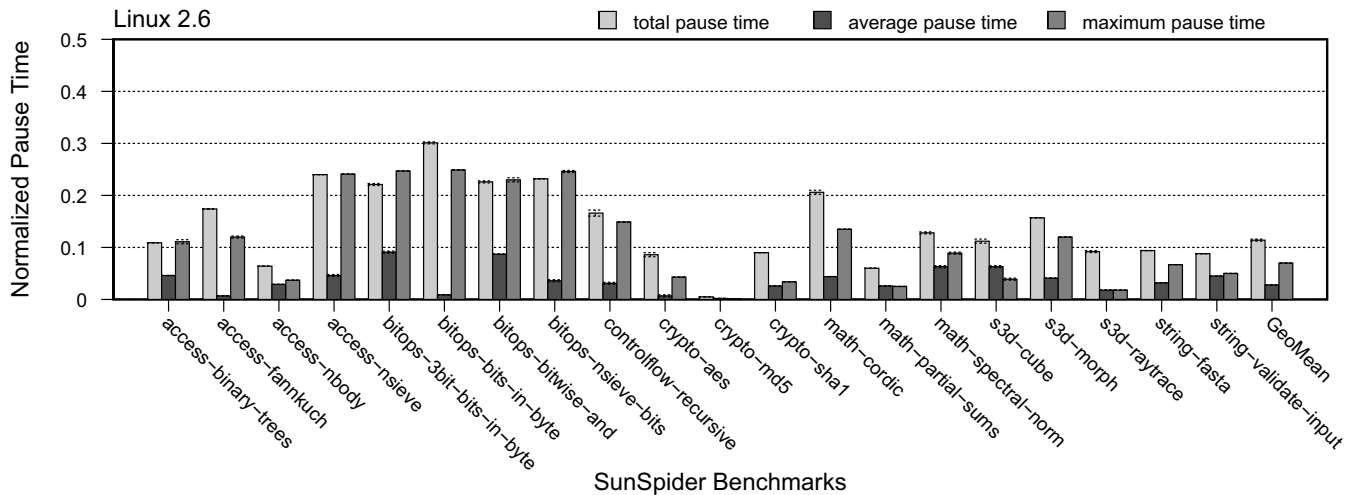
Figure 4. Pause time ratios of concurrent vs. sequential JITs.
