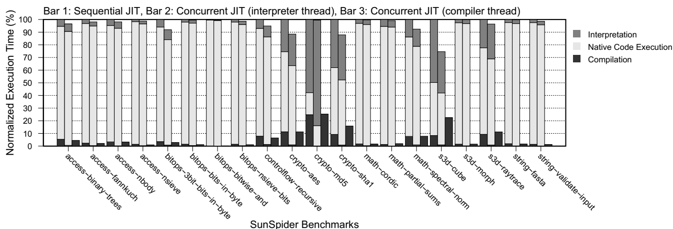
Figure 5. Execution time improvements. Average time is break down in compilation, native code, and interpretation.
