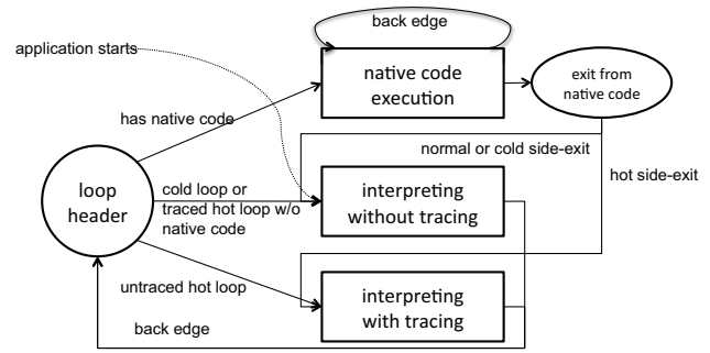
Figure 3. The interpreter state transition at a loop header.
