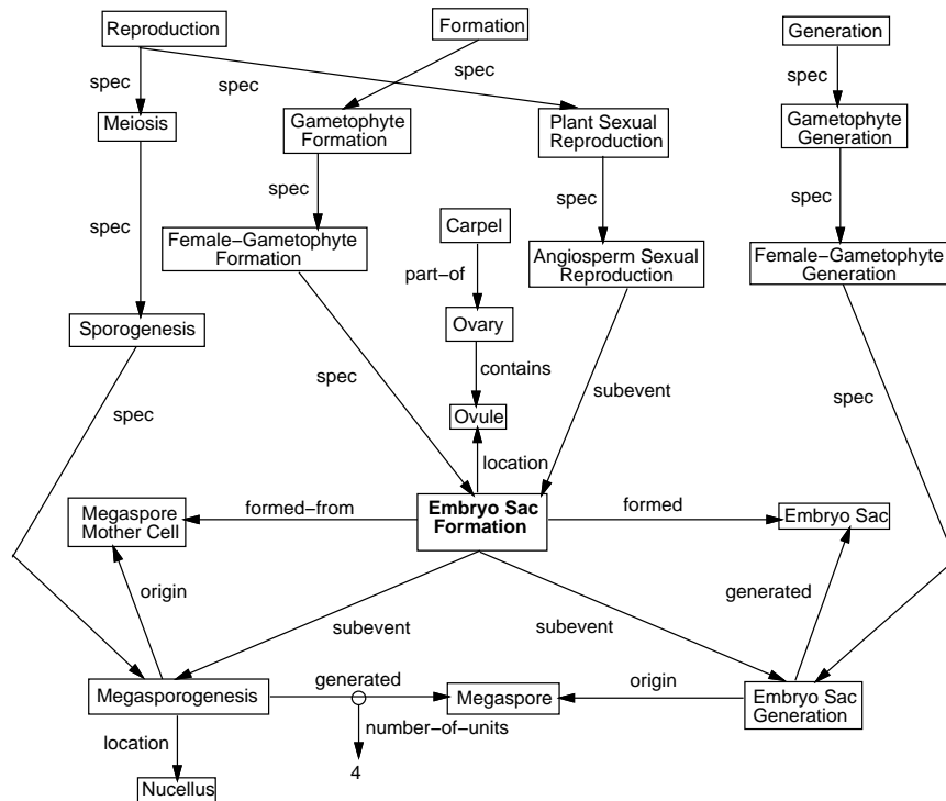
Figure 13: A representation of embryo sac formation
