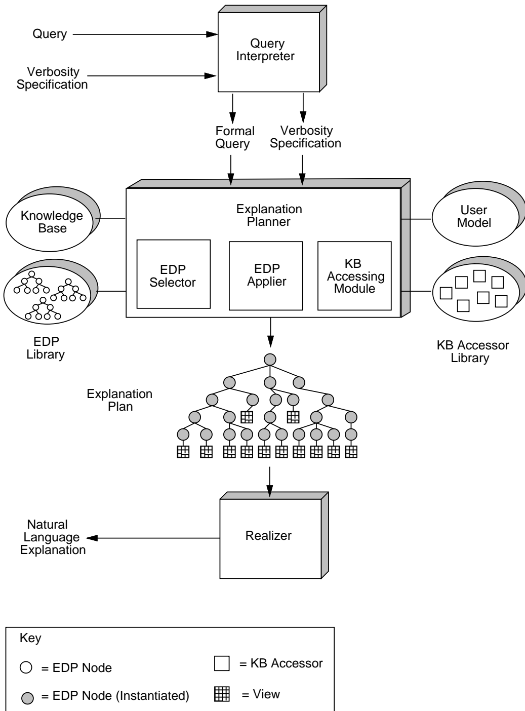
Figure 9: An Architecture for Explanation Generation
