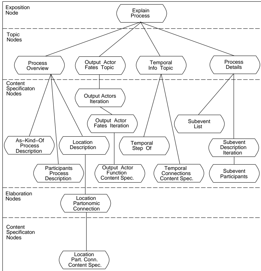
Figure 8: The Final Version of the Explain-Process Explanation Design
