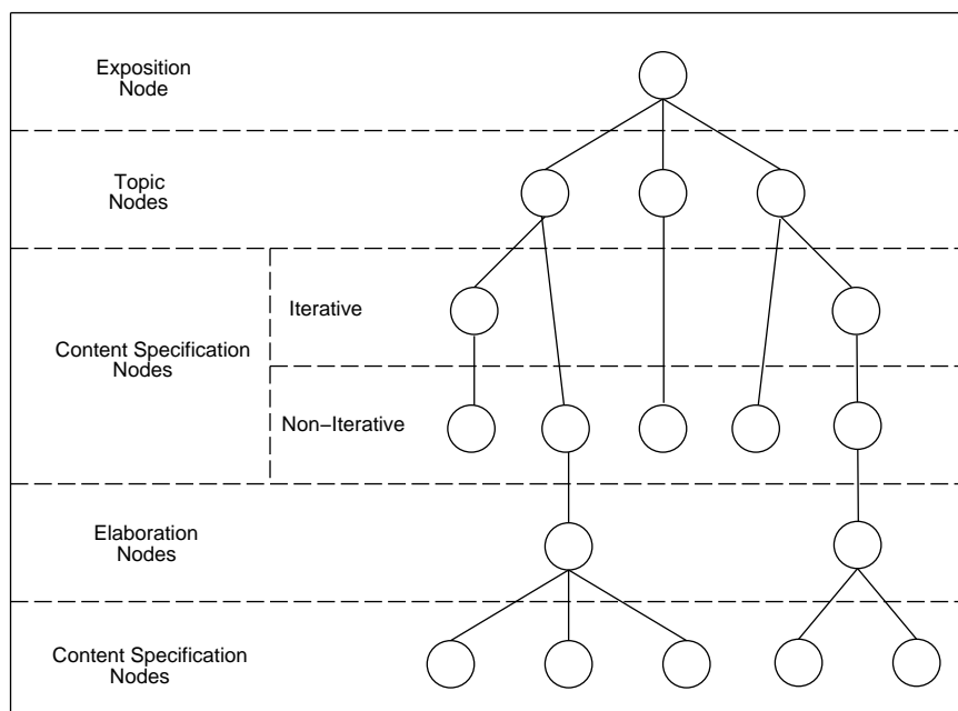
Figure 6: The Layers of Explanation Design Packages
