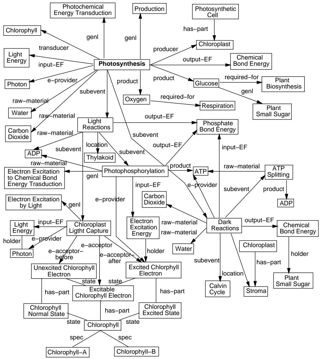
Figure 3: A sample representational structure from the Biology Knowledge Base
