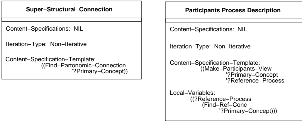
Figure 7: Example content specification nodes
