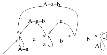
Figure 1: Finite State Machine to recognize the substring “abb”
