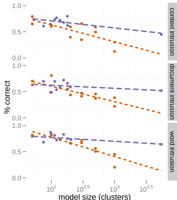
Figure 5: Scatterplot of model size vs. avg score for MVM (dashed, purple) and LDA (dotted, orange); Syntax+Documents data.
