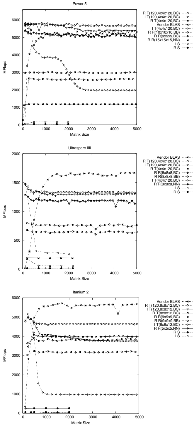
Figure 4: Complete MMM performance
