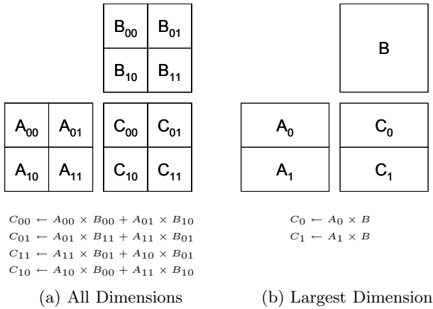
Figure 3: Divide-and-conquer strategies for MMM
