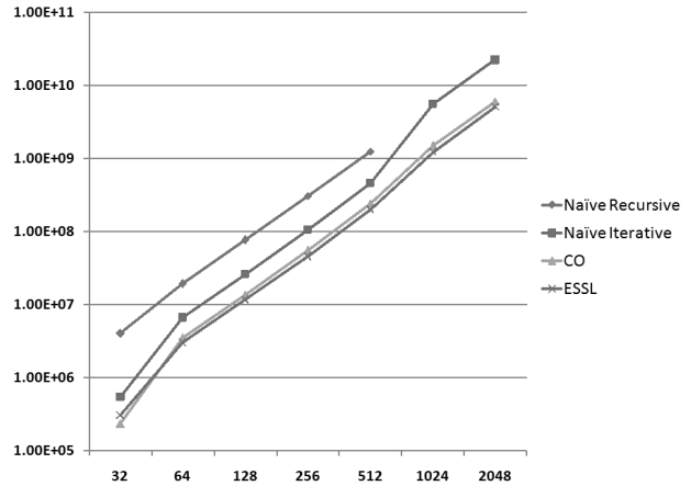
Figure 10: Matrix Transpose runtime in cycles on IBM Blue Gene for all four implementations using square matrices (log scale).
