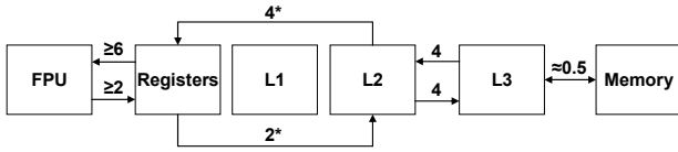
Figure 2: Bandwidth of the Itanium 2 memory hierarchy, measured in doubles/cycle 3 .
