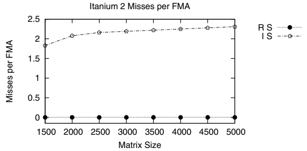
Figure 5: Data cache misses per FMA instruction in MMM
