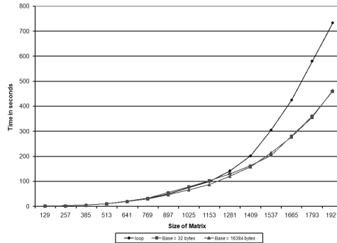
Figure 1: An empirical study of recursive and iterative matrix multiplication programs
