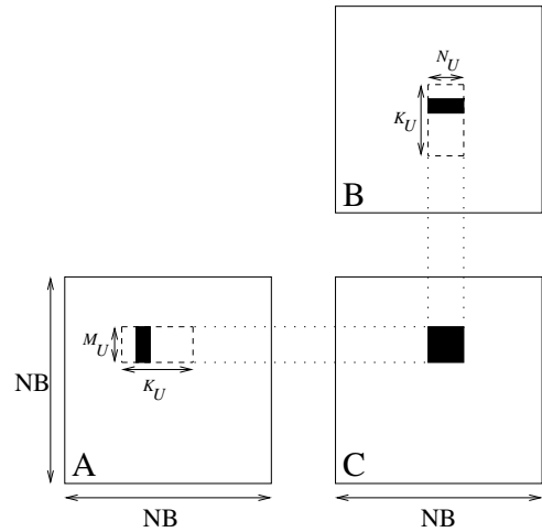
Figure 9: Iterative microkernel and minikernel used in ATLAS
