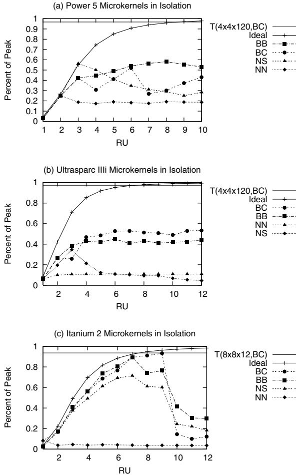
Figure 6: Microkernel performance in isolation
