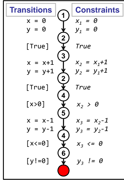
Fig. 9. Abstract Counterexample
