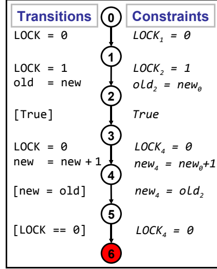
Fig. 7. Abstract Counterexample
