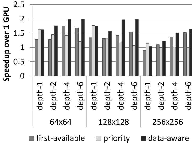
Figure 12: Speedup of PTask using 2 GTX580 GPUs over PTask using 1 GTX580 GPU, for a range of graph sizes using matrix multiplication ptasks. Data for the fifo scheduling policy is omitted because it is similar to that for first-available.
