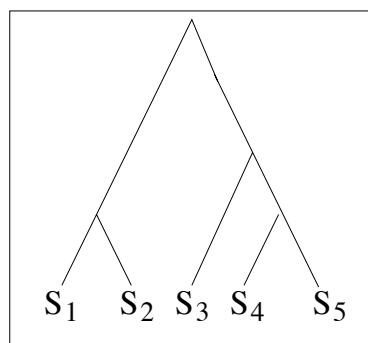
TRUE TREE
