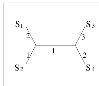
INFERRED TREE
