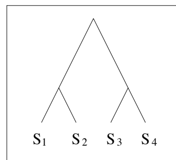
TRUE TREE
