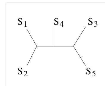
INFERRED TREE
