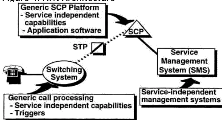
Figure 4. AIN Architecture
