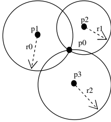
Figure 7. An Example of Trilateration
