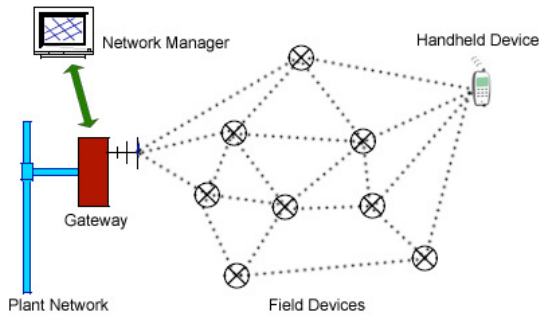
Figure 1. A Typical WirelessHART Network
