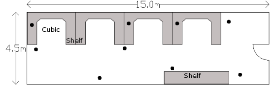
Figure 8. Indoor Testbed
