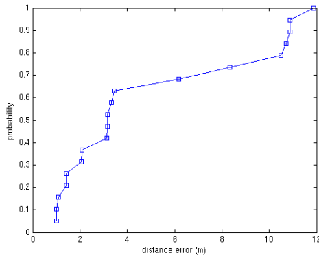
Figure 13. Distance Error CDF(outdoor)
