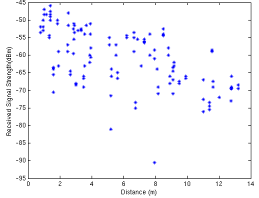
Figure 6. Actual Distances and Received Signal Strength
