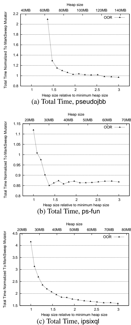
Figure 13: Garbage Collection vs. Idealized Mark-Sweep
