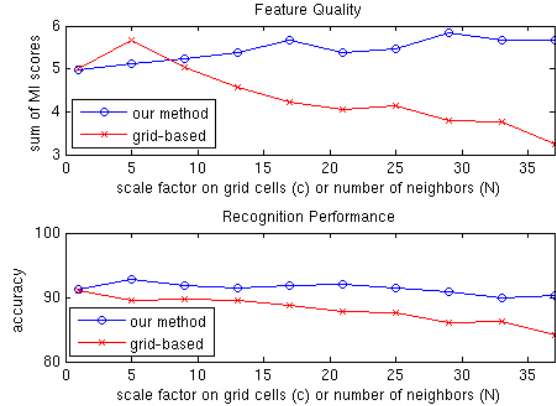
Figure 7. Top: Distinctiveness of the neighborhood (level-1) visual words for our features and a grid-based baseline. Bottom: Recognition results for the same two methods. Note that a single x , y , t weight combination is used here. See text for details.
