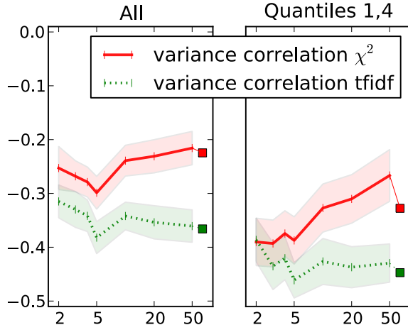
Figure 4: Plots of variance correlation; lower numbers indicate higher negative correlation, i.e. that prototype entropy predicts rater disagreement.
