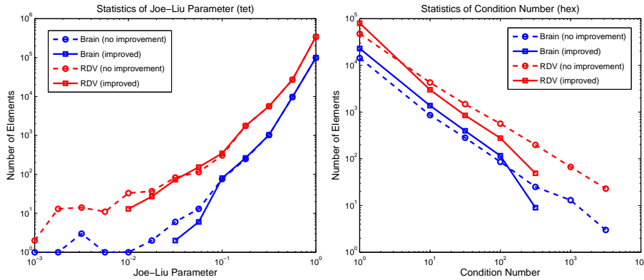
Fig. 13. The histogram of Joe-Liu parameter (left) of tet hexes, and the condition number (right) of hex meshes for the human brain and the RDV data. It is obvious that the mesh quality, especially the worst parameter, is improved
