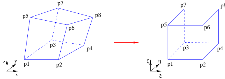
Fig. 11. A hexahedron [p1p2...p8] is mapped into a trilinear parametric volume in terms of \xi , \eta , and \zeta . The eight basis functions in Equation (4) are attached to the eight vertices of the hexahedron.
