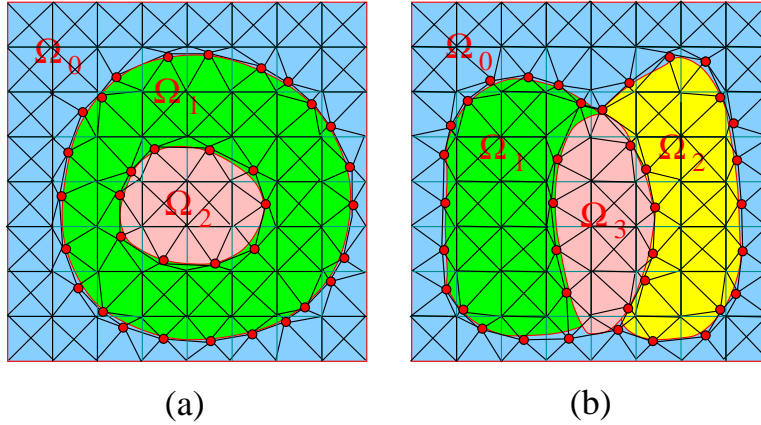
Fig. 5. 2D triangulation for a domain with multiple materials. (a) - there are three materials, and \cup B_i constructs manifold curves; (b) - there are four materials, and \cup B_i constructs non-manifold curves and a square outer boundary.
