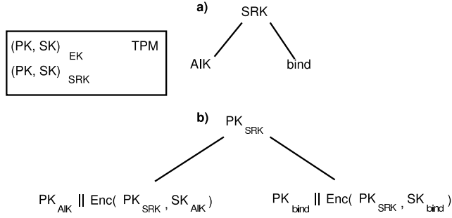
Figure 3: The part of the TPM key hierarchy relevant to our attack. The TPM box illustrates keying material stored internal to the TPM, which is only the endorsement key (EK) and storage root key (SRK). Part (a) shows the conceptual key hierarchy, while part (b) shows how the secret keys of children are encrypted by the public keys of their parents so keys can be safely stored in memory. More detail on key formats is found in Figure 2.
