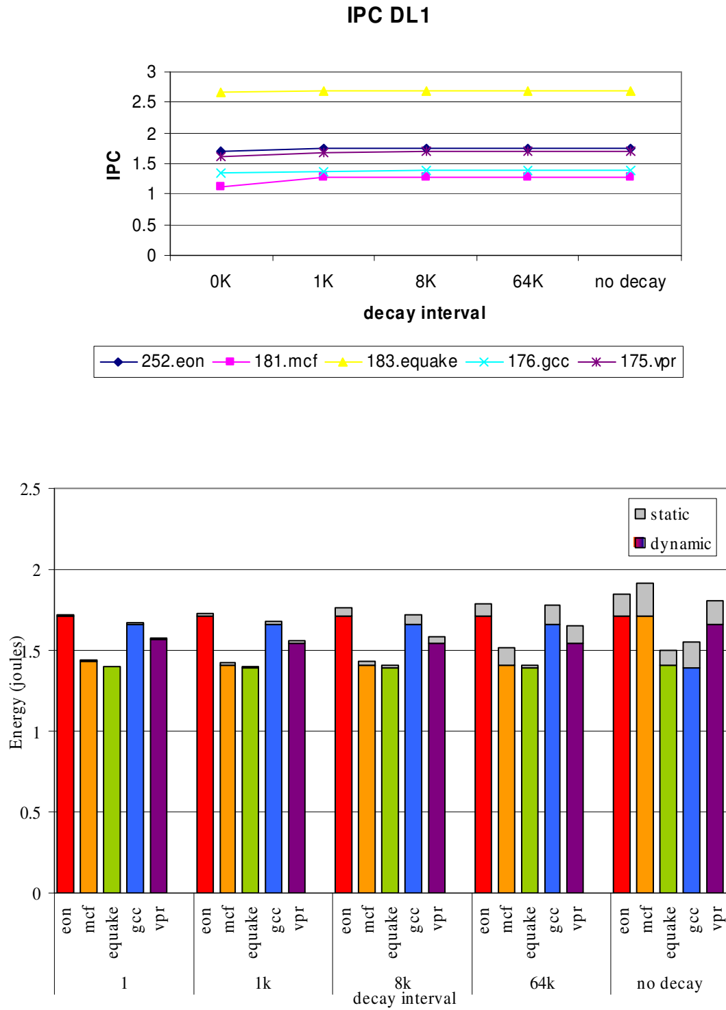
Figure 21: MTCMOS Level-1 Data Cache Measurements
