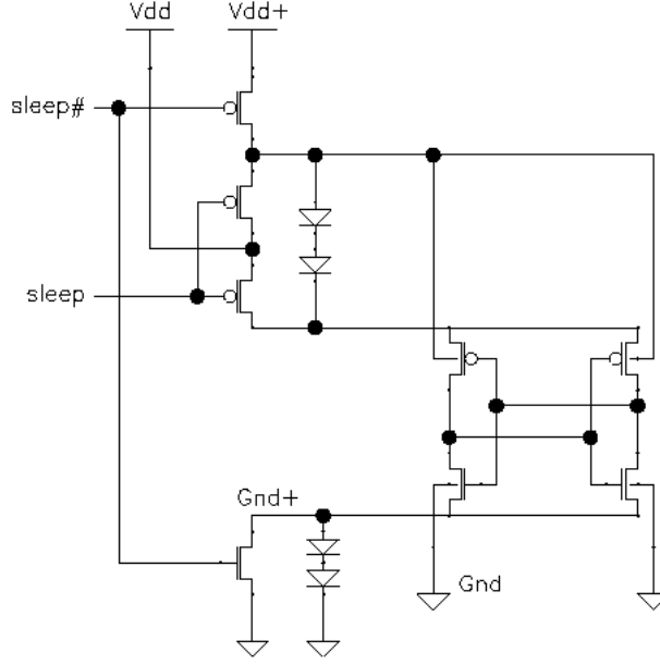
Figure 9 MTCMOS schematic
