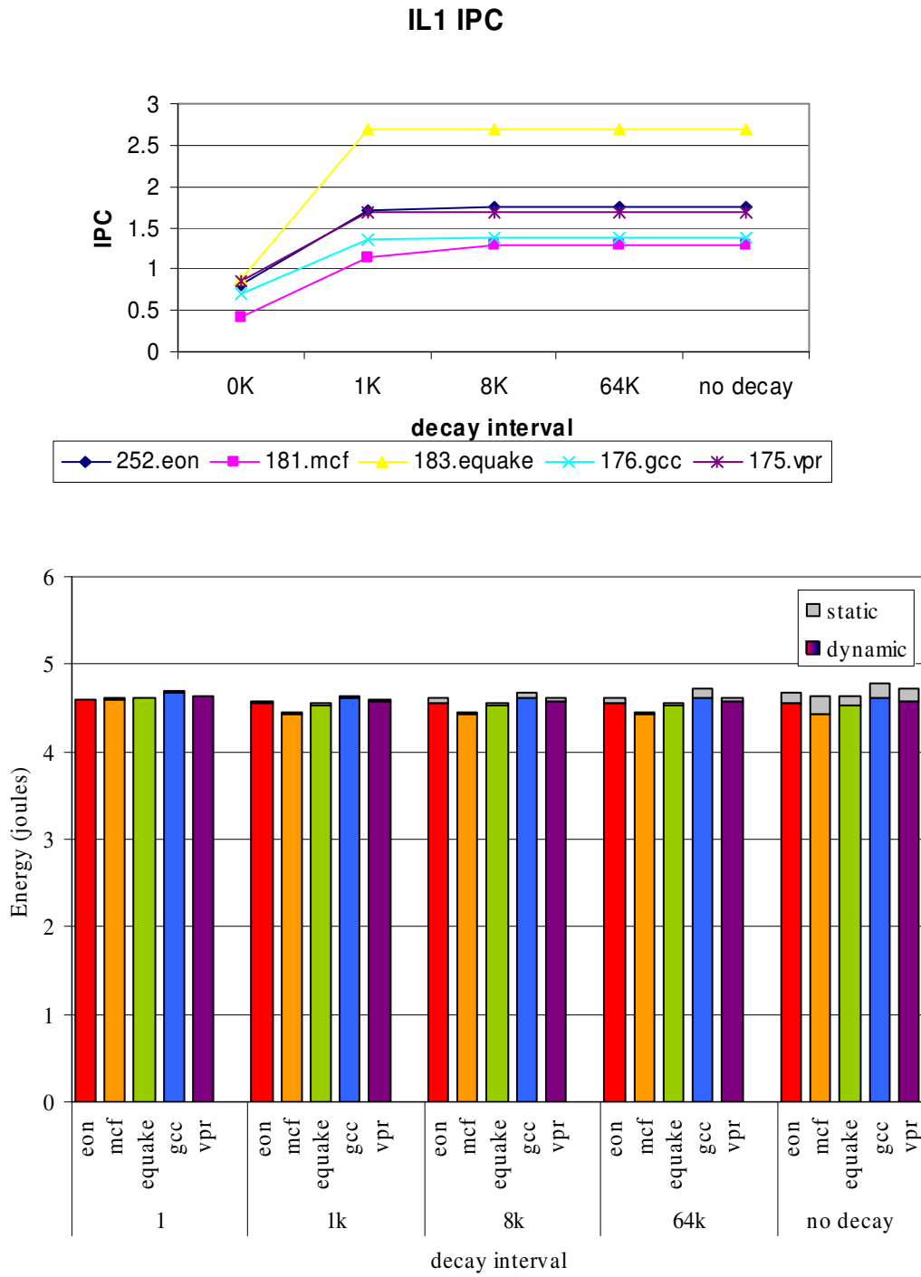
Figure 20: MTCMOS Level-1 Instruction Cache Measurements
