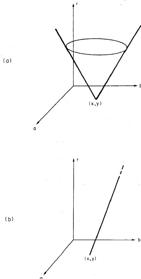
Fig. 2. (a) Locus of parameters with no directional information. (b) Locus of parameters with directional information.
