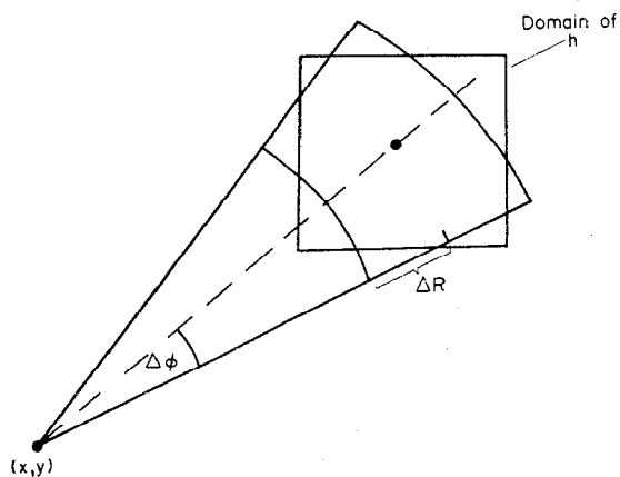
Fig. 3. Using convolution templates to compensate for errors.
