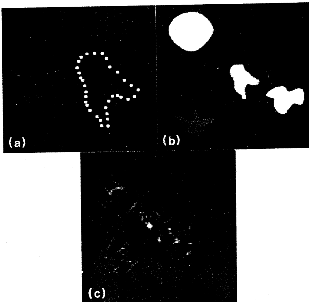
Fig. 8. An example. (a) Points on a shape used to encode R -table. (b) Image containing shape. (c) A plane through the accumulator array A(x_r, y_r, S_0, \theta_0) , where S_0 and \theta_0 are appropriate for the shape in the image ( S_0 = 64, \theta_0 = 0 ).
