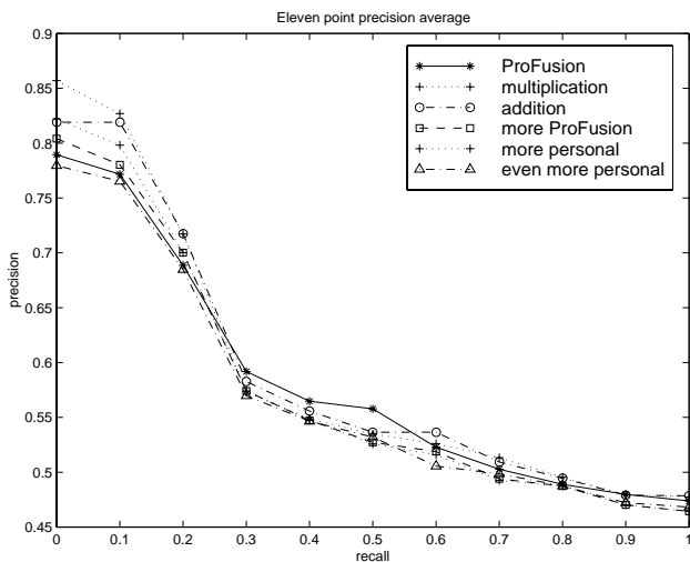
Figure 3. 11 point average precision for interest adjustment function \Delta \iota(c_i) = \log \frac{time}{\log(\log length)} \cdot \gamma(d, c_i) and 5 different ranking formulae.
