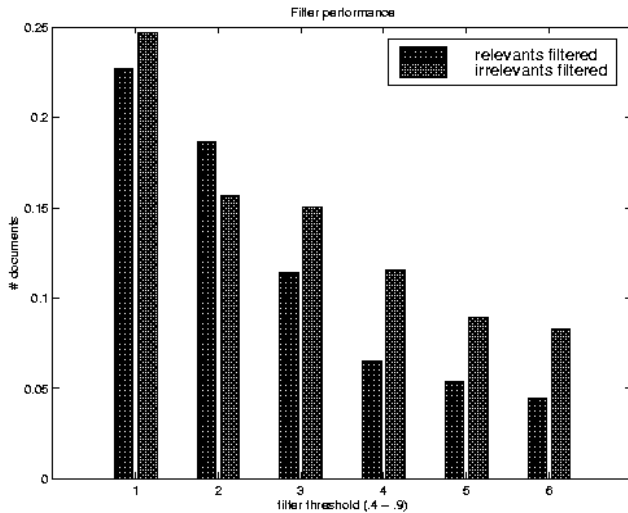
Figure 5. Average filter performance: Training. Adjustment function \Delta t(c_i) = \log \frac{time}{\log length} \cdot \gamma(d, c_i) . Abscissa: threshold values from .4 to .9; ordinate: ratio of relevant (non-relevant) documents.
