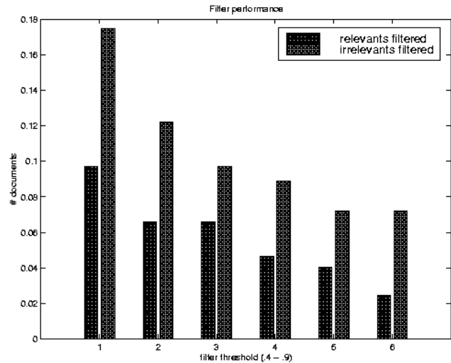
Figure 6. Average filter performance: Testing. Adjustment function \Delta t(c_i) = \log \frac{time}{\log length} \cdot \gamma(d, c_i) . Abscissa: threshold values from .4 to .9; ordinate: ratio of relevant (non-relevant) documents.
