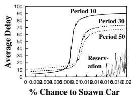
Fig. 4: Average delays for traffic light systems with period 10, 30, and 50 seconds plotted against varying traffic levels along with a 1-tiled reservation-based system.
