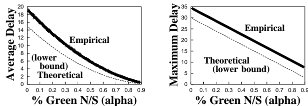
Fig. 3. Average (left) and maximum (right) delay as a function of \alpha for 1,000,000 steps of the simulation, spawning cars with probability .001.
