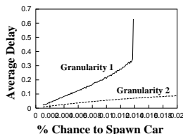
Fig. 5: The average delay for granularity 1 and 2 reservation systems with varying traffic levels. Each data point represents 1,000,000 steps of simulation.
