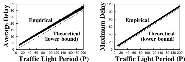
Fig. 2. Average (left) and maximum (right) delay as a function of P for 1,000,000 steps of the simulation, spawning cars with probability .002.
