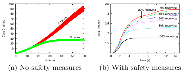
Figure 2: Average crash logs (2(a) includes 95% confidence interval) with and without safety measures. In 2(a), both the 3- and 6-lane scenarios are shown. In 2(b), 0, 20, 40, 60, 80, and 100% of vehicles receive the Emergency-Stop message.
