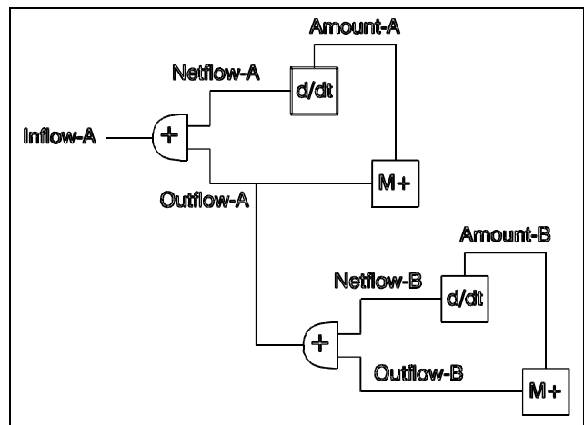
Figure 3. Correct model for cascaded tanks.
