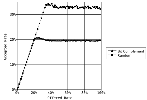
Fig. 4. Accepted traffic versus offered traffic as a percentage of maximum input bandwidth for bit-complement and random traffic
