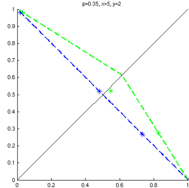
Figure 4: Inconsistency of Cross Entropy The distribution is supported on u = (1, x) and v = (y, 1) with probability p and 1-p respectively. The 3 green points are G(u)/\|G(u)\|_D , G(v)/\|G(v)\|_D and their weighted mean. The 3 blue points are \exp(u)/\mathbf{1}^\top \exp(u) , \exp(v)/\mathbf{1}^\top \exp(v) and their weighted mean. Note that the weighted means lie on different sides of the black diagonal line.
