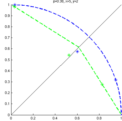
Figure 3: Inconsistency of Cosine The distribution is supported on u = (1, x) and v = (y, 1) with probability p and 1-p respectively. The 3 green points are G(u)/\|G(u)\|_D , G(v)/\|G(v)\|_D and their weighted mean. The 3 blue points are G(u)/\|G(u)\|_2 , G(v)/\|G(v)\|_2 and their weighted mean. Note that the weighted means lie on different sides of the black diagonal line.
