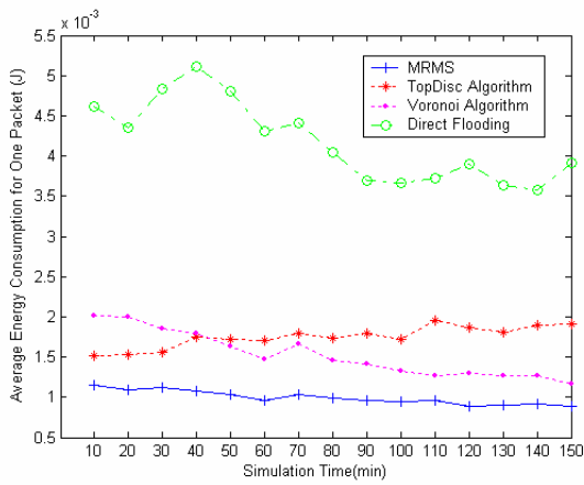
Figure 8. Average Energy Consumption for packet
