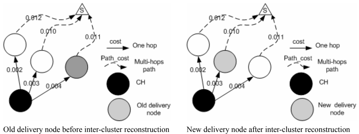
Figure 4. Changing Delivery Node in Cluster Reconstruction
