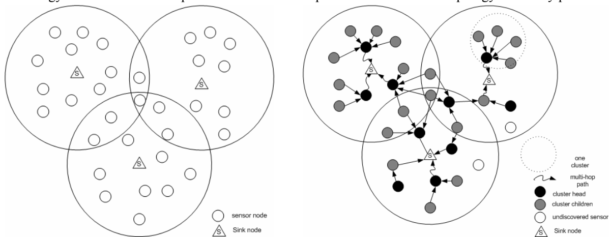
(a) Sensor and sink nodes before topology discovery (b) Sensor and sink nodes after topology discovery
