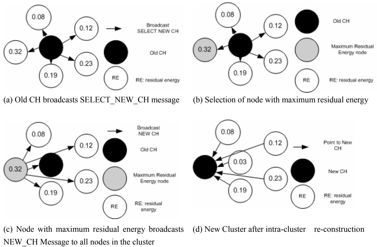
Figure 3. Intra-Cluster Reconstruction
