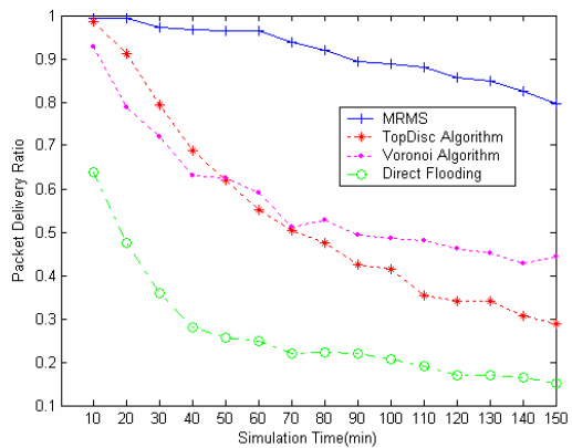
Figure 11. Packet Delivery Ratio
