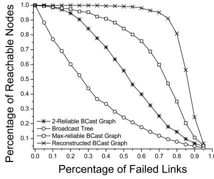
Fig. 19. Reachability in broadcast graphs
