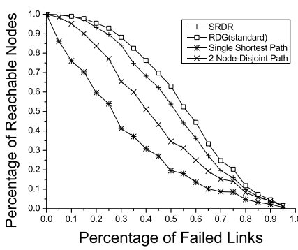
Fig. 22. Reachability in downlink graph
