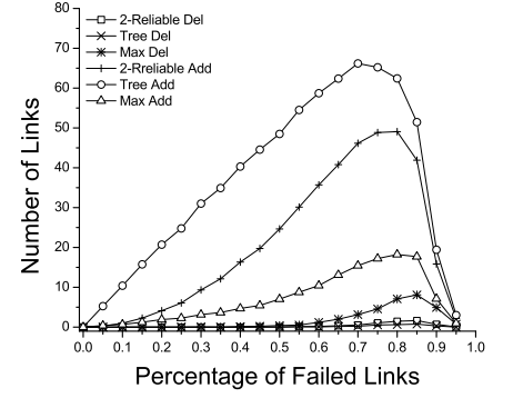
Fig. 20. Recovery overhead to regain connectivity
