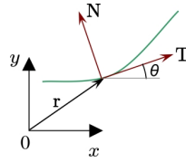
Fig. 5. Tangent and Normal to a curve.
