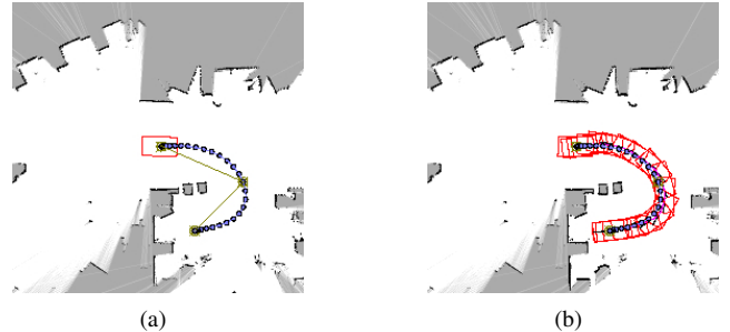
Fig. 7. (a) A real world example of a comfortable trajectory. This trajectory is composed of several sub-goals, given by a trivial RRT planner. (b) Actual path of the robot. A static feedback linearization controller [10] is used to compute the control commands necessary to follow the trajectory.
