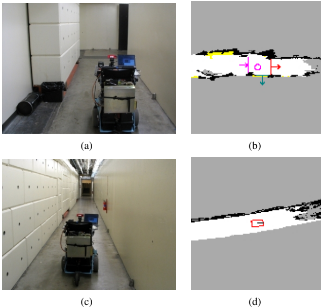
Fig. 12. (a) Texture-less walls (e.g., the solid wall at the right of this image) often lead to poor distance information from the stereo camera. (b) This causes gaps in the wall when it is modeled in the vision-based LPM. This leads to incorrect gateways and to false positive place detections in the environment. (c) A particular wall that is often completely invisible to stereo. (d) This leads to an LPM with a large boundary between free and unknown regions, which results in no gateways being found. Thus, the wheelchair has no way to autonomously travel down this hallway in the current implementation.
