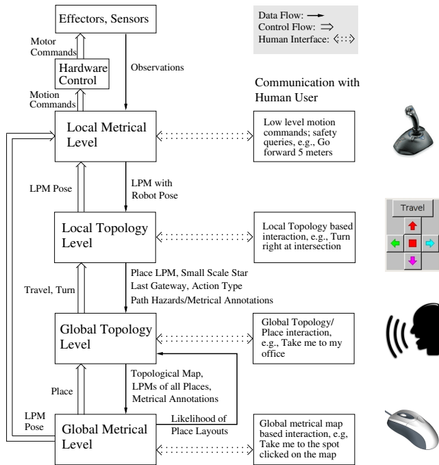
Fig. 2. The cognitive architecture of the Intelligent Wheelchair is based on the HSSH. The rightmost column shows the interface modes we are currently investigating for each representational level.
