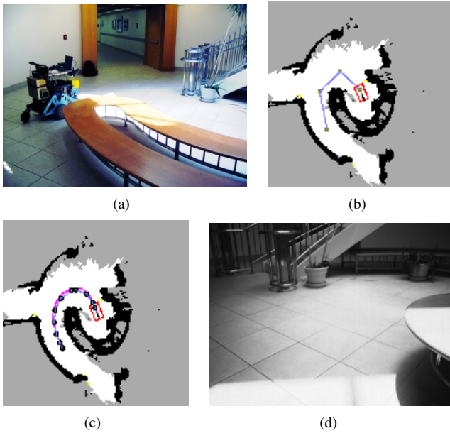
Fig. 9. (a,b) The stereo camera is able to detect an overhanging bench top that cannot be seen by the wheelchair’s horizontal lidar. Thus, in this scenario the vision-based LPM provides a useful model for safe planning. (c) The wheelchair computes a trajectory that results in a smooth path and comfortable motion by using the vision-based LPM. (d) A snapshot from the robot’s camera as it navigates around the bench.
