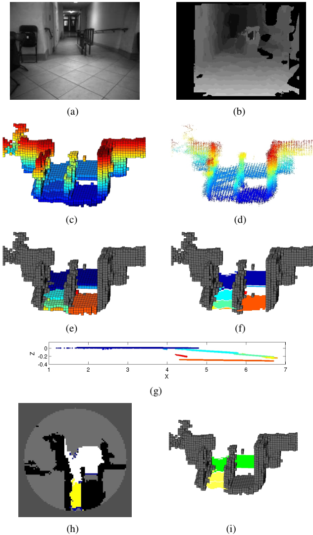
Fig. 4. (Best viewed in color) (a) Left image from the stereo camera showing a typical non-planar scene, with a drop-off to the left, and a ramp to the right, of the railing. (b) Disparity map computed for the stereo pair (brighter regions closer). (c) 3D occupancy grid of the above environment (voxels colored according to height) constructed from a collection of stereo images. (For clarity, the viewpoint of this figure is different from the viewpoint of the left image above.) (d) 3D point cloud that built the occupancy grid. (e) Potentially traversable ground regions found by segmenting the 3D grid. (Obstacles are gray.) (f) The planes obtained for each of the potential ground segments. (g) A cross-sectional view of the planes. (h) The final safety map obtained after analyzing the segments and fitted planes for safety: black for Non-ground regions; white for Level regions; yellow for Inclined regions; light gray for Unknown regions; dark gray for unexamined regions; and blue for denoting Potential Drop-off Edges that might be present in the Level and Inclined regions. (i) A hybrid 3D model can also be constructed at this point. The planes are used to represent traversable ground regions (green for Level and yellow for Inclined regions). The grid is used to represent Non-ground regions that are not modeled easily using planes.
