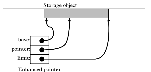
Figure 1: Modified pointer representation: pointer-base-address-extent triple
