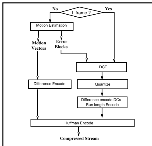
Figure 3 : The MPEG compression algorithm
