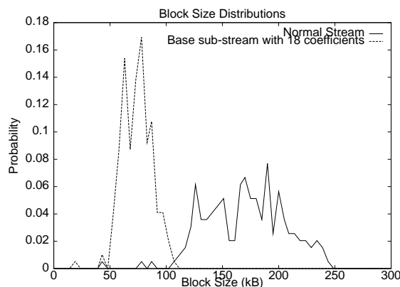
Figure 9 : Comparison of block size distribution of the base sub-stream with the normal stream
