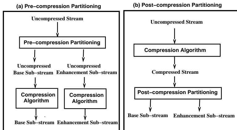
Figure 2 : Temporal partitioning techniques
