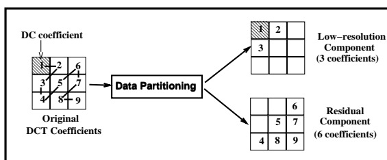
Figure 4 : The data partitioning technique
