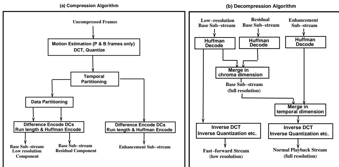
Figure 5 : The compression and decompression algorithms
