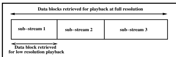
Figure 1 : Contiguous placement of sub-stream blocks
