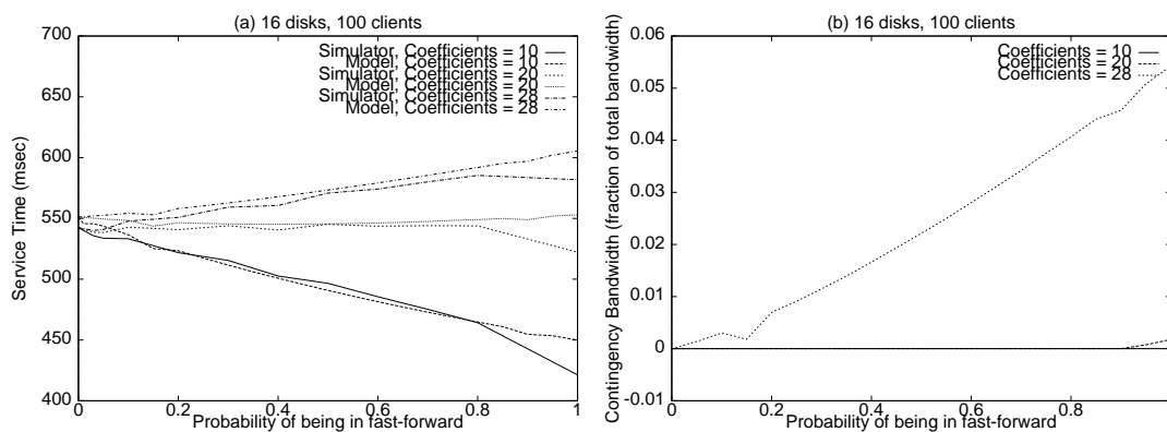
Figure 10 : Variation in service times and the contingency bandwidth obtained by changing the probability of fast-forward.
