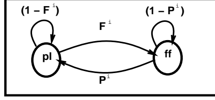
Figure 6 : The Markov model for the behavior of a client
