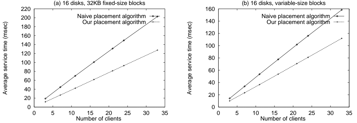
Figure 7 : Service time of a disk during normal playback: Our placement algorithm yields a smaller service time per disk as compared to one that interleaves each sub-stream independently across the array.
