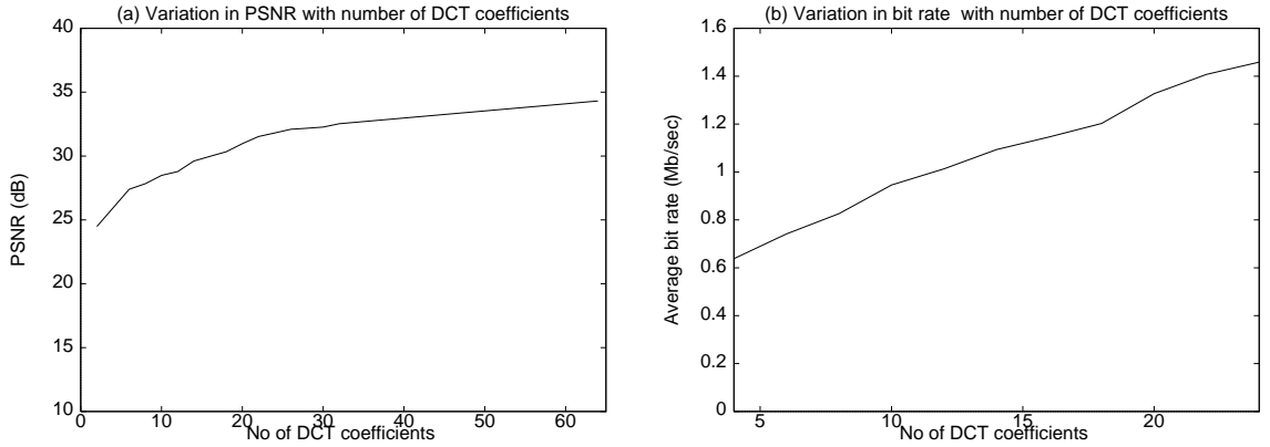
Figure 8 : Variation of PSNR and fast-forward bit rates with number of DCT coefficients for the Frasier sequence.
