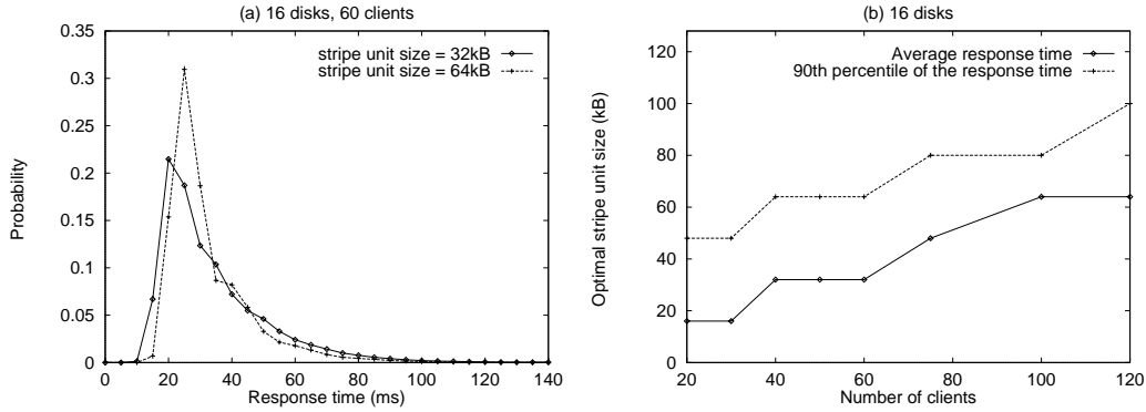
Figure 1: Effect of different metrics on the stripe unit size.
