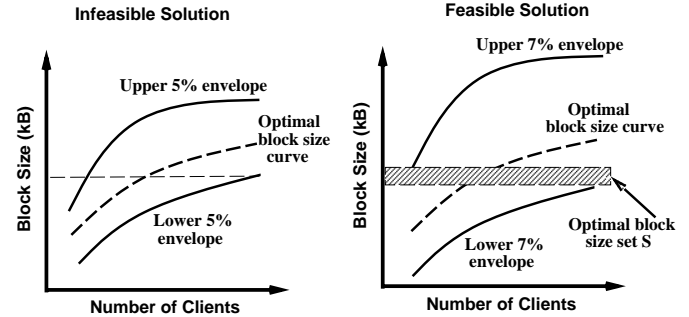
Figure 7: Selecting a block size that yields near-optimal performance, regardless of the number of clients accessing the server. The shaded region denotes the set of block sizes S that yield service times within 7% of the minimum for all workloads.
