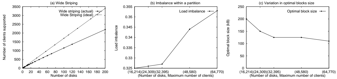
Figure 8: Loss in the number of clients supported in large disk arrays and factors contributing to this loss.
