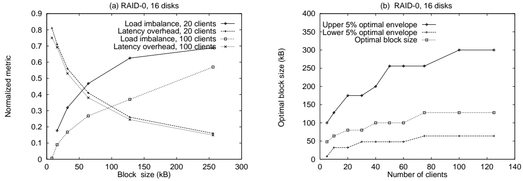
Figure 6: Effect of number of clients on the optimal block size.
