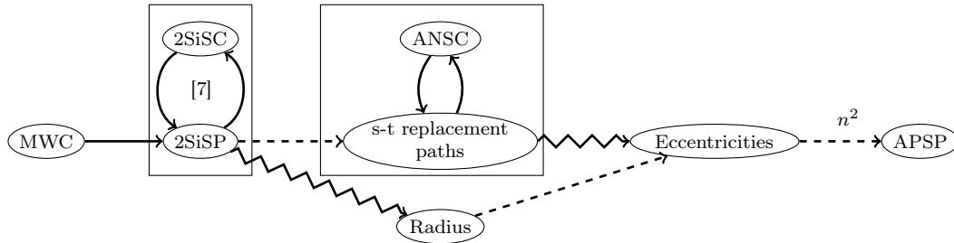
Figure 1: Our sparse reductions for weighted directed graphs (reductions related to centrality problems are in Figure 8). The regular edges represent sparse O(m + n) reductions, the squiggly edges represent tilde-sparse \tilde{O}(m + n) reductions, and the dashed edges represent reductions that are trivial. The n^2 label on dashed edge to APSP denotes an O(n^2) time reduction.
