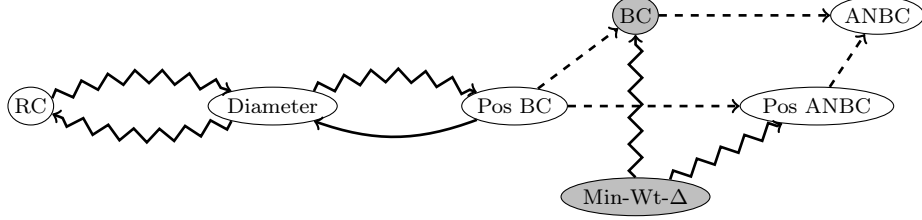
Figure 7: Known sparse reductions for centrality problems, all from [3]. The regular edges represent sparse O(m+n) reductions, the squiggly edges represent tilde-sparse O(m+n) reductions, and the dashed edges represent reductions that are trivial. BC and Min-Wt- \Delta (shaded with gray) are known to be sub-cubic equivalent to APSP [3, 42].
