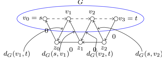
Figure 6: G' for l = 3 in the reduction: directed s - t Replacement Paths \leq_{m+n}^{\text{spr s}} \text{ANSC}
