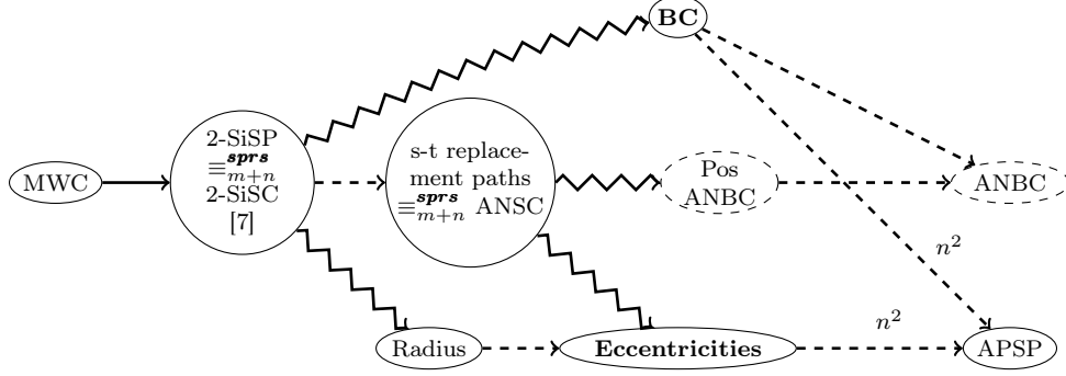
Figure 8: Sparse reductions for weighted directed graphs. The regular edges represent sparse O(m + n) reductions, the squiggly edges represent tilde-sparse O(m + n) reductions, and the dashed edges represent reductions that are trivial. All problems except APSP are MWCC-hard. Eccentricities, BC, ANBC and Pos ANBC are also SETH/ k -DSH hard. ANBC and Pos ANBC (problems inside the dashed circles) are both not known to be subcubic equivalent to APSP.
