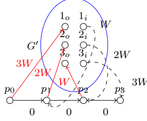
Figure 5: G' for n = 3 in the reduction: directed \text{MWC} \leq_{m+n}^{\text{spr s}} 2\text{-SiSP}
