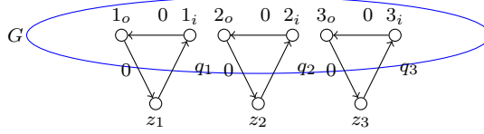
Figure 10: G' for n = 3 in the reduction: directed \text{ANSC} \lesssim_{m+n}^{\text{spr}s} \text{Pos ANBC} .
