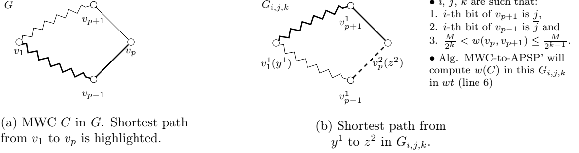
Figure 4: Here Figure (a) represent the MWC C in G . The path \pi_{y,z} (in bold) is the shortest path from y to z in G . The path \pi_{y^1,z^2} (in bold) in Figure (b) is the shortest path from y^1 to z^2 in G_{i,j,k} : where the edge (v_{p-1}^1, v_p^2) is absent due to i, j bits. The paths \pi_{y,z} in G and \pi_{y^1,z^2} in G_{i,j,k} together comprise the MWC C .
