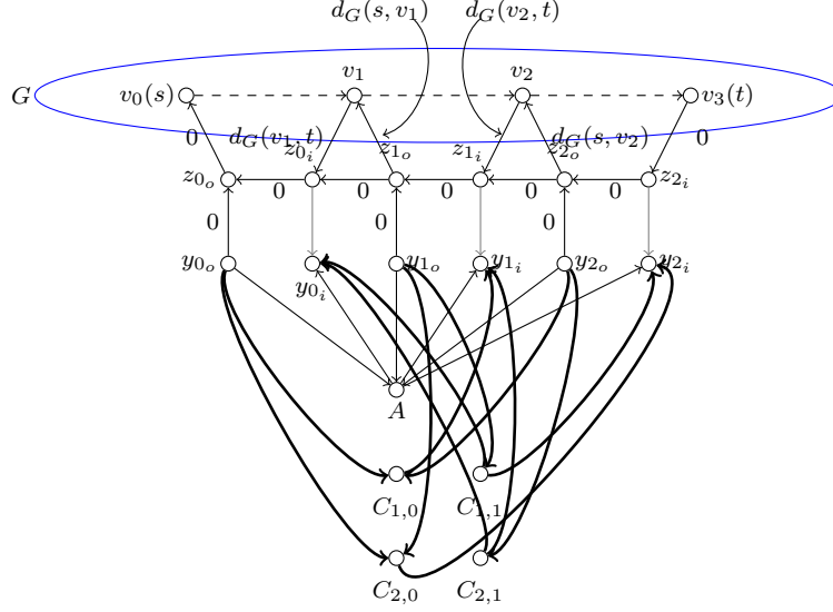
Figure 9: G'' for l = 3 in the reduction: directed 2-SiSP \stackrel{\text{spr}s}{\sim}_{m+n} Betweenness Centrality. The gray and the bold edges have weight M' and \frac{1}{3}M' respectively. All the outgoing (incoming) edges from (to) A have weight M' + q(0) .
