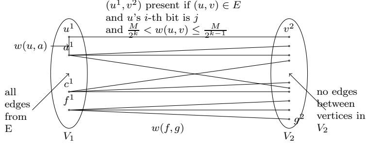
Figure 2: Construction of G_{i,j,k} .
