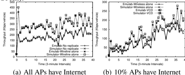
Figure 9: Cross validation: comparing performance in Emulab and simulation
