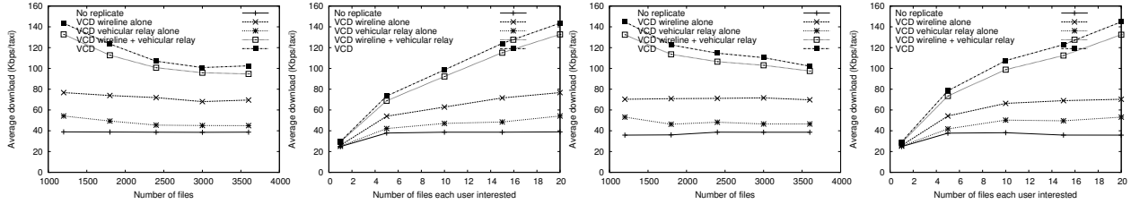
(a) Uniform: vary # files (b) Uniform: vary # files per user (c) Zipf-like: vary # files (d) Zipf-like: vary # files per user
