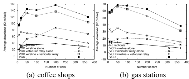
Figure 7: Average throughput under a varying number of vehicles (San Francisco, Zipf-like traffic, range = 100m).
