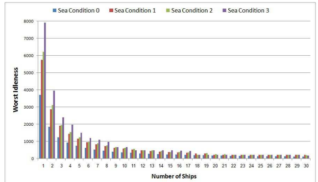
Figure 3: The worst idleness returned from Algorithm HeuristicDivide in the four different sea conditions examined.
