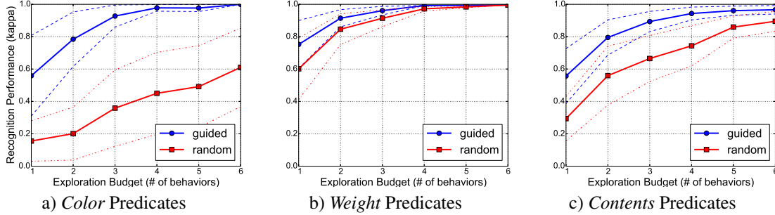
Figure 2: Test-time \kappa performance of classifiers for learning a new predicate based on the reliability weight estimation strategy used at test time as more behaviors are allowed. random chooses the next exploratory behavior at random, while guided uses word embeddings to select known neighbor predicates from which to estimate reliability weights for behaviors. The dotted lines denote the variance over 75 simulation runs.
