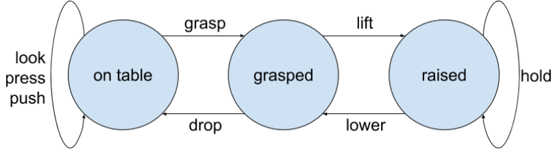
Figure 7: Exploratory behavior actions as transitions in an object state graph.
